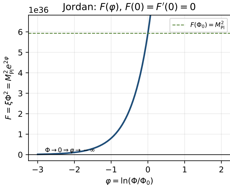
Fig.3 Domain-wall / EFT boundary at \Phi = 0 (two frames)
