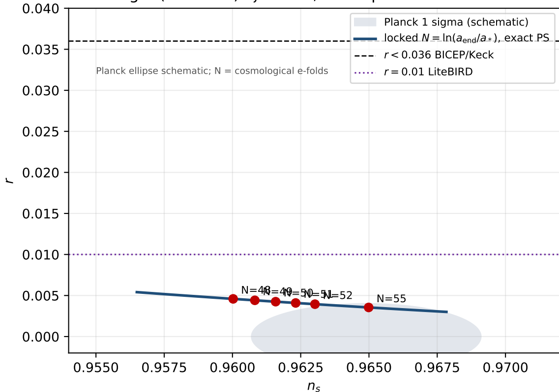
Fig.2 (locked N ) \xi = 11.1 , exact potential slow-roll
