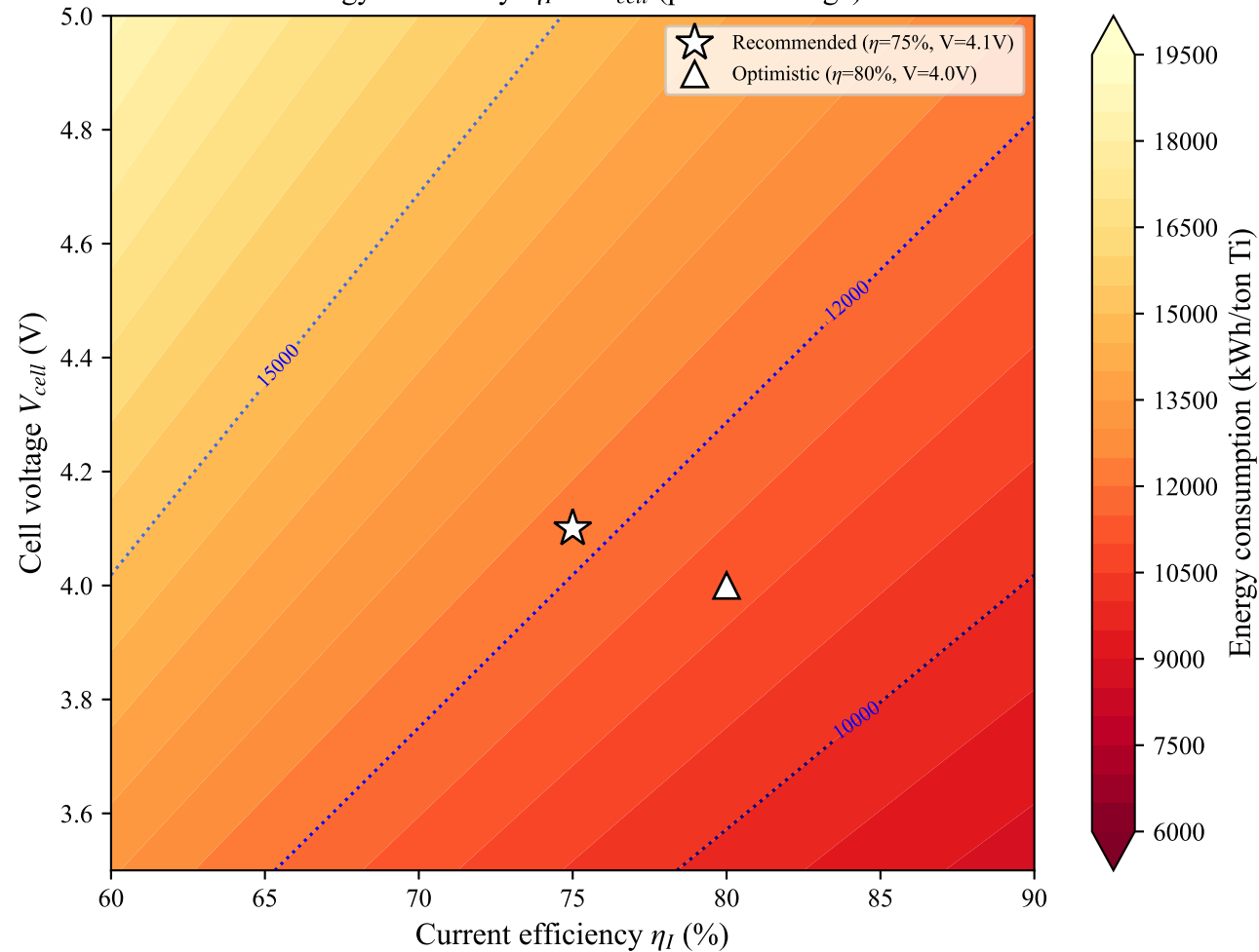
Energy Sensitivity: \eta_I vs V_{cell} (practical range)
