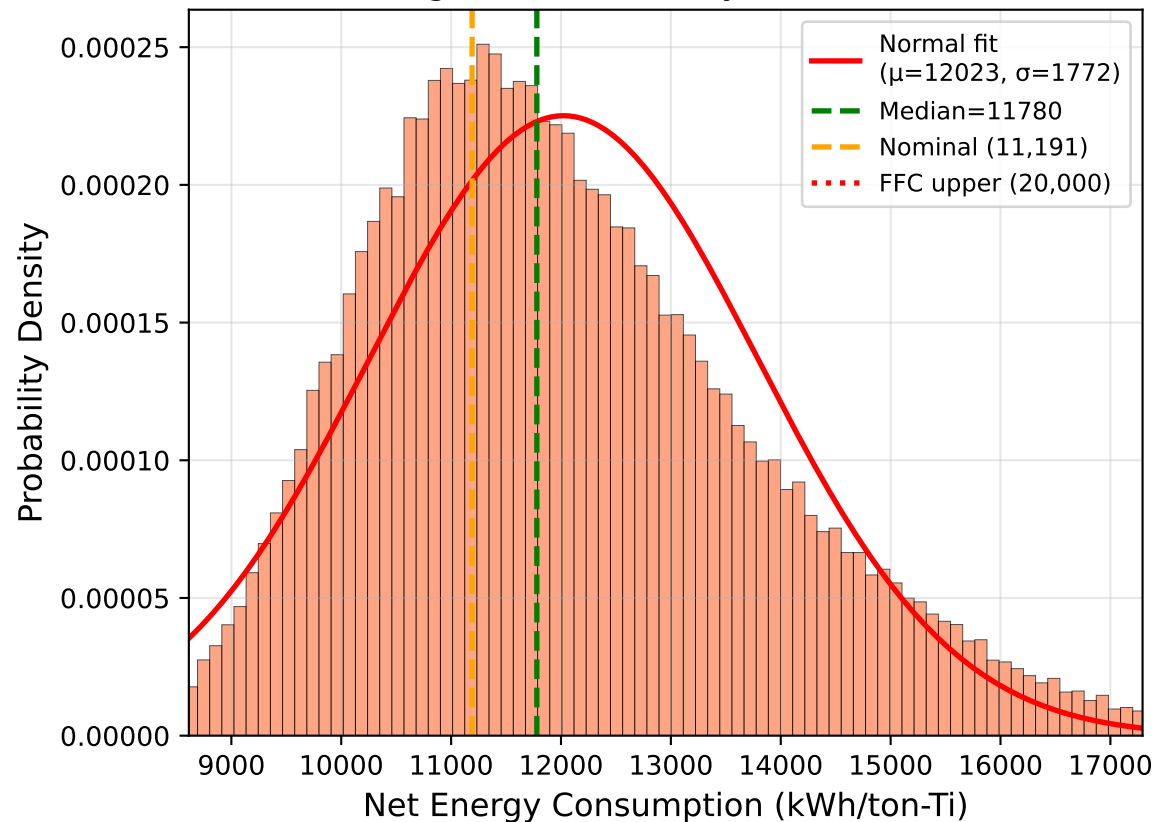
Net Energy Consumption Distribution (global uncertainty, N=100k)
