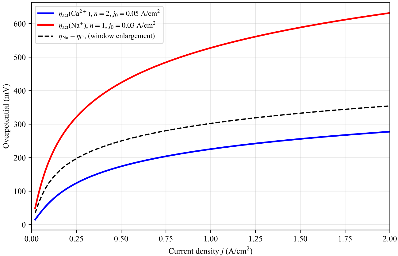
Butler-Volmer Activation Overpotential vs Current Density (600 °C, \alpha = 0.5 , order-of-magnitude j_0 )
