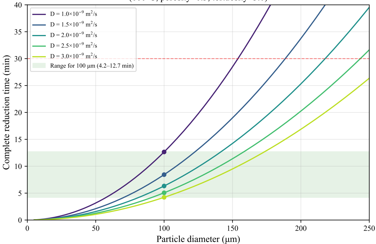
SCM Sensitivity: Reduction Time vs D (600°C, porosity=0.3, tortuosity=3.0)
