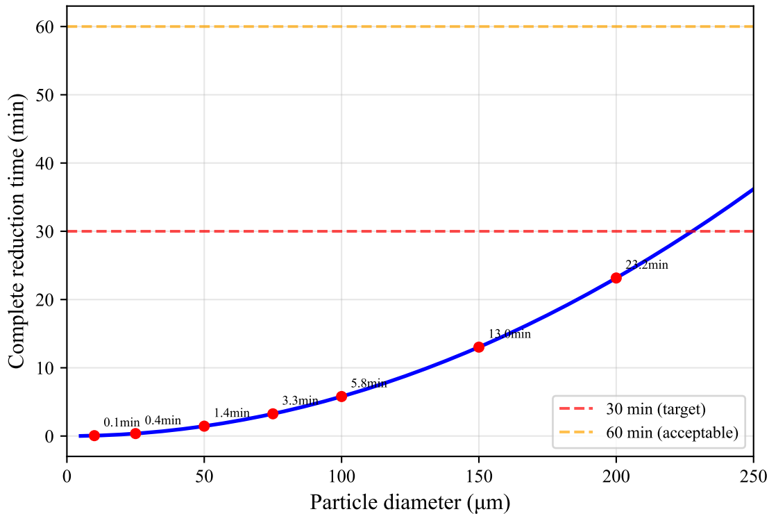
Complete Reduction Time vs Particle Size (Diffusion-controlled SCM, 600°C)
