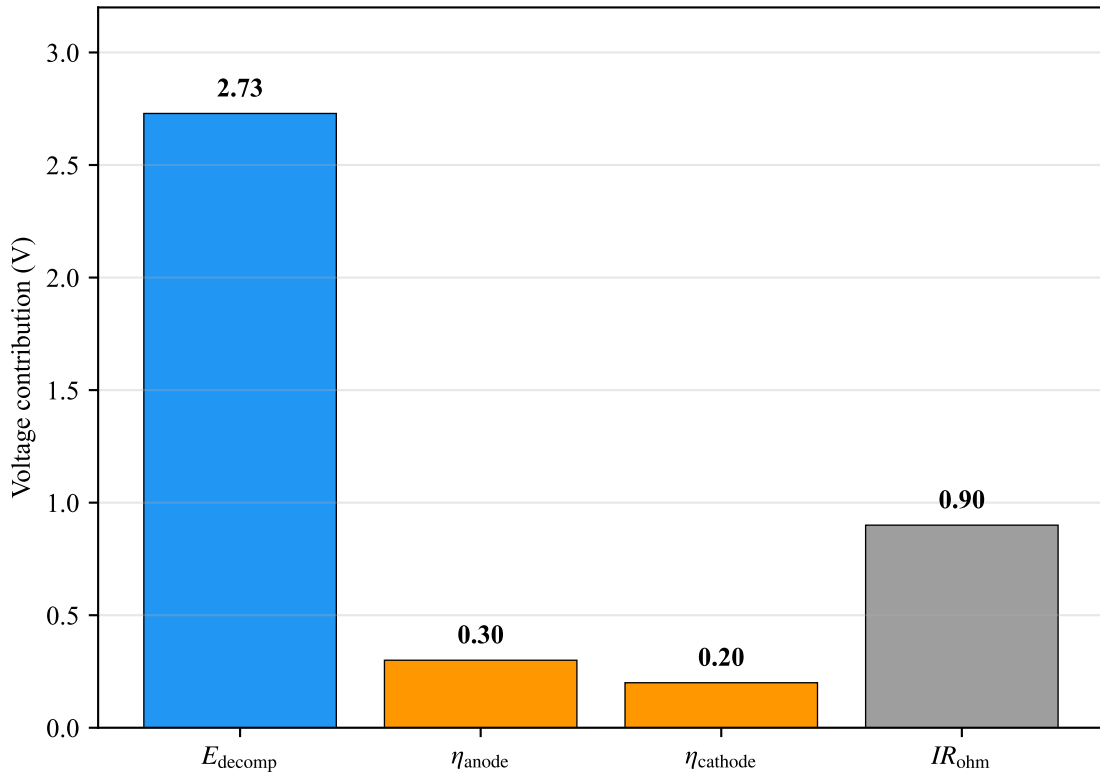
Cell Voltage Decomposition (600 °C, order-of-magnitude)
