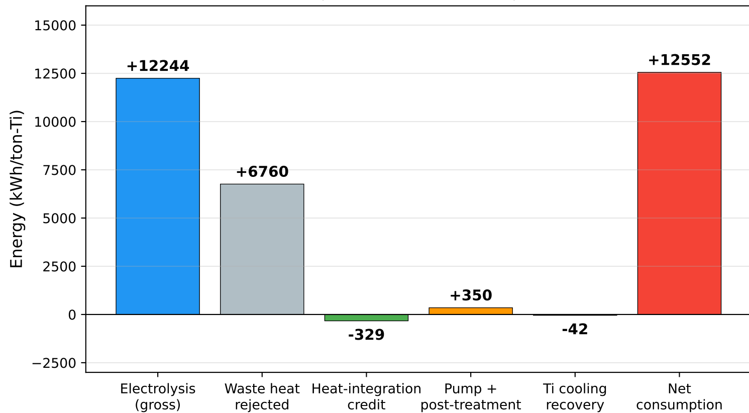
Revised Heat Balance: Energy Flow Breakdown (basis: 1 ton Ti, 600°C)
