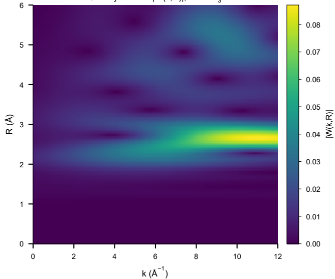
Cauchy wavelet |W(k,R)| , Pt foil L_3
