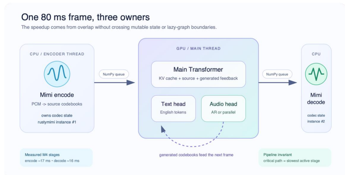
Figure 1 — Streaming architecture: one 80 ms frame, three owners (measured M4 stages: encode ~17 ms, decode ~16 ms).
