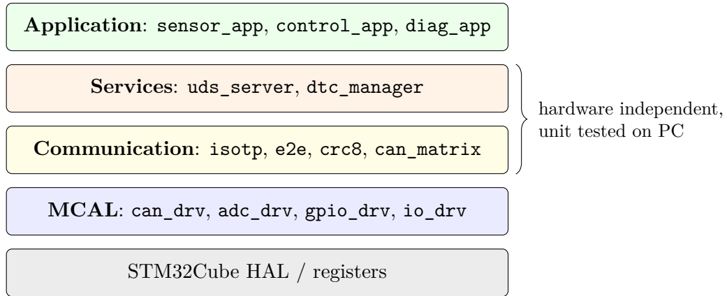
Figure 3.2: AUTOSAR-inspired software layers
