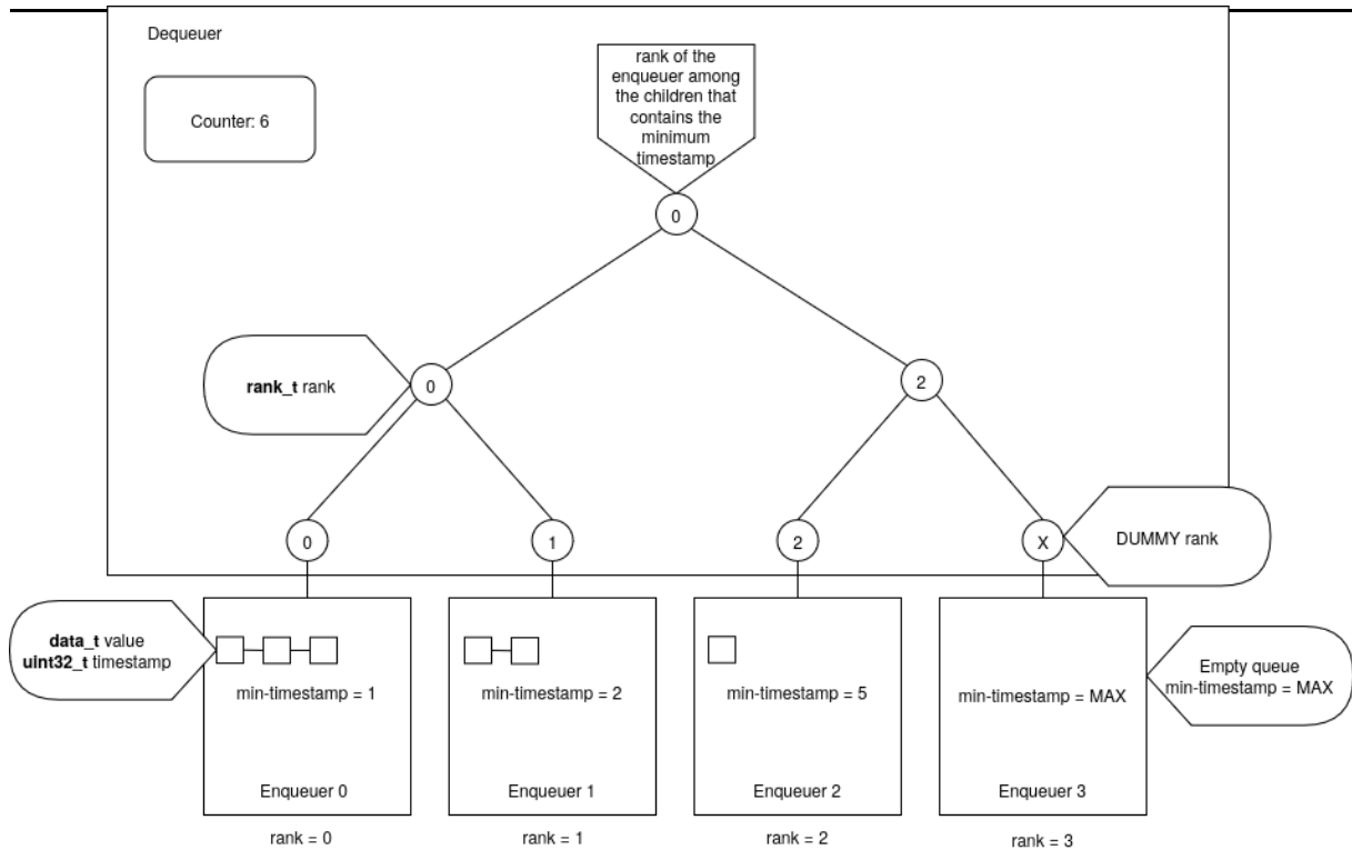
Figure 18: dLTQueue's structure.
