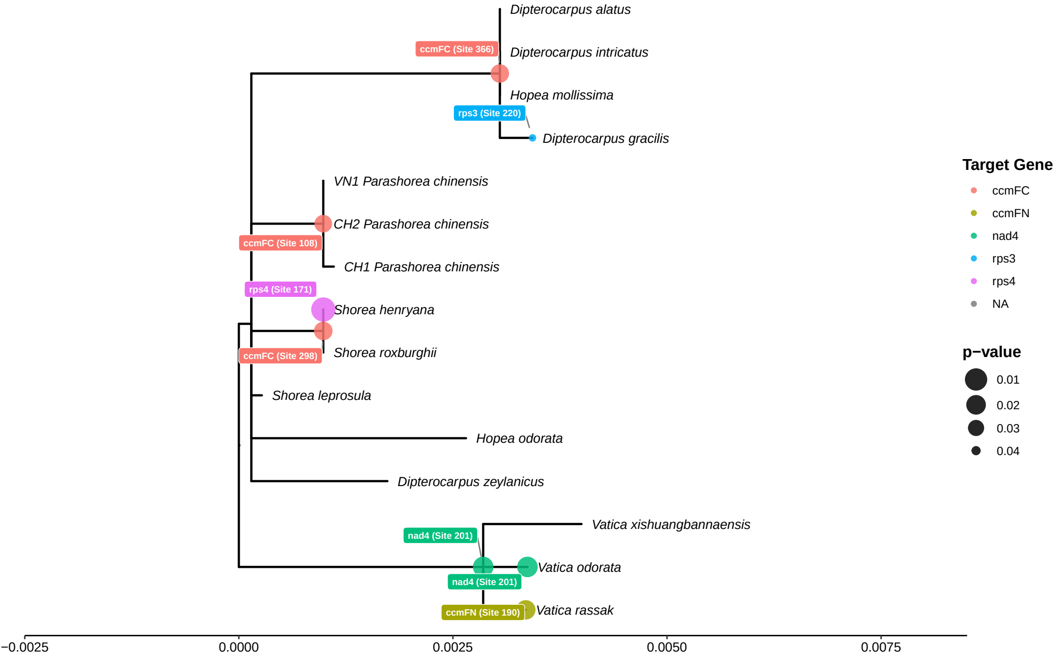
Phylogenetic Distribution of Episodic Positive Selection (HyPhy MEME)
