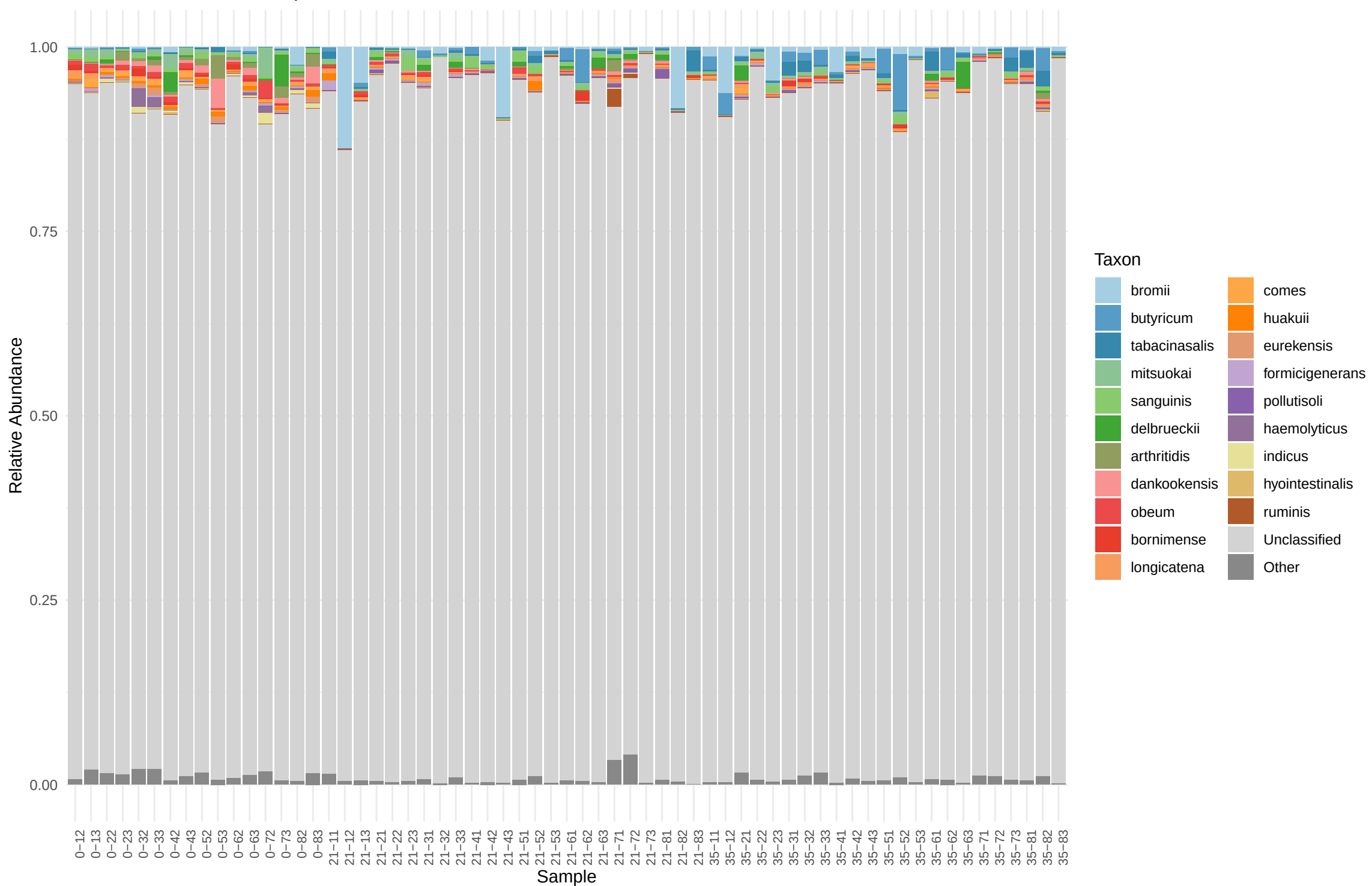
Relative Abundance at Species Level
