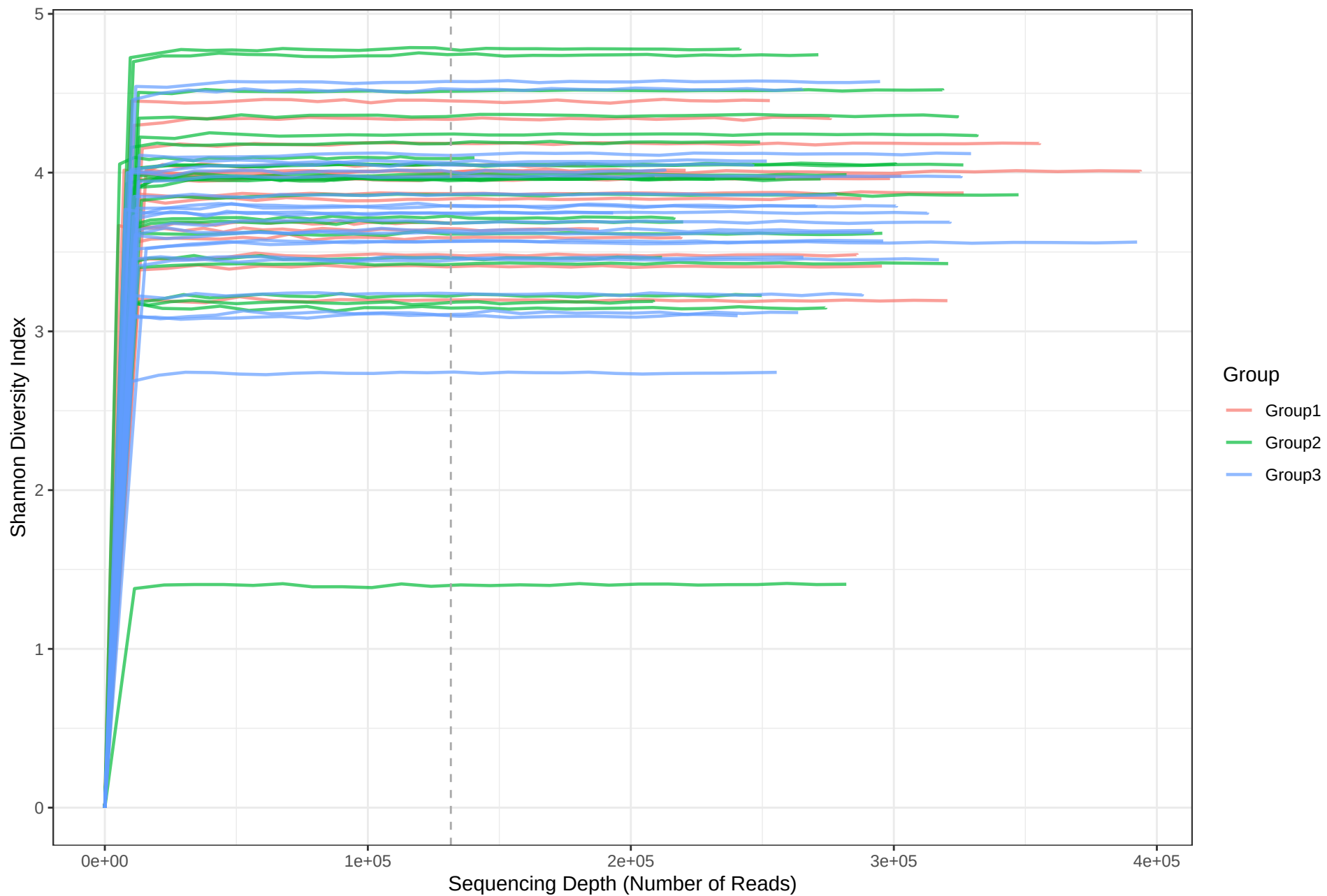
ASV-Level Shannon Diversity Saturation
