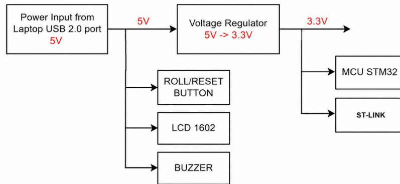
Figure 3.4: Power tree for components
