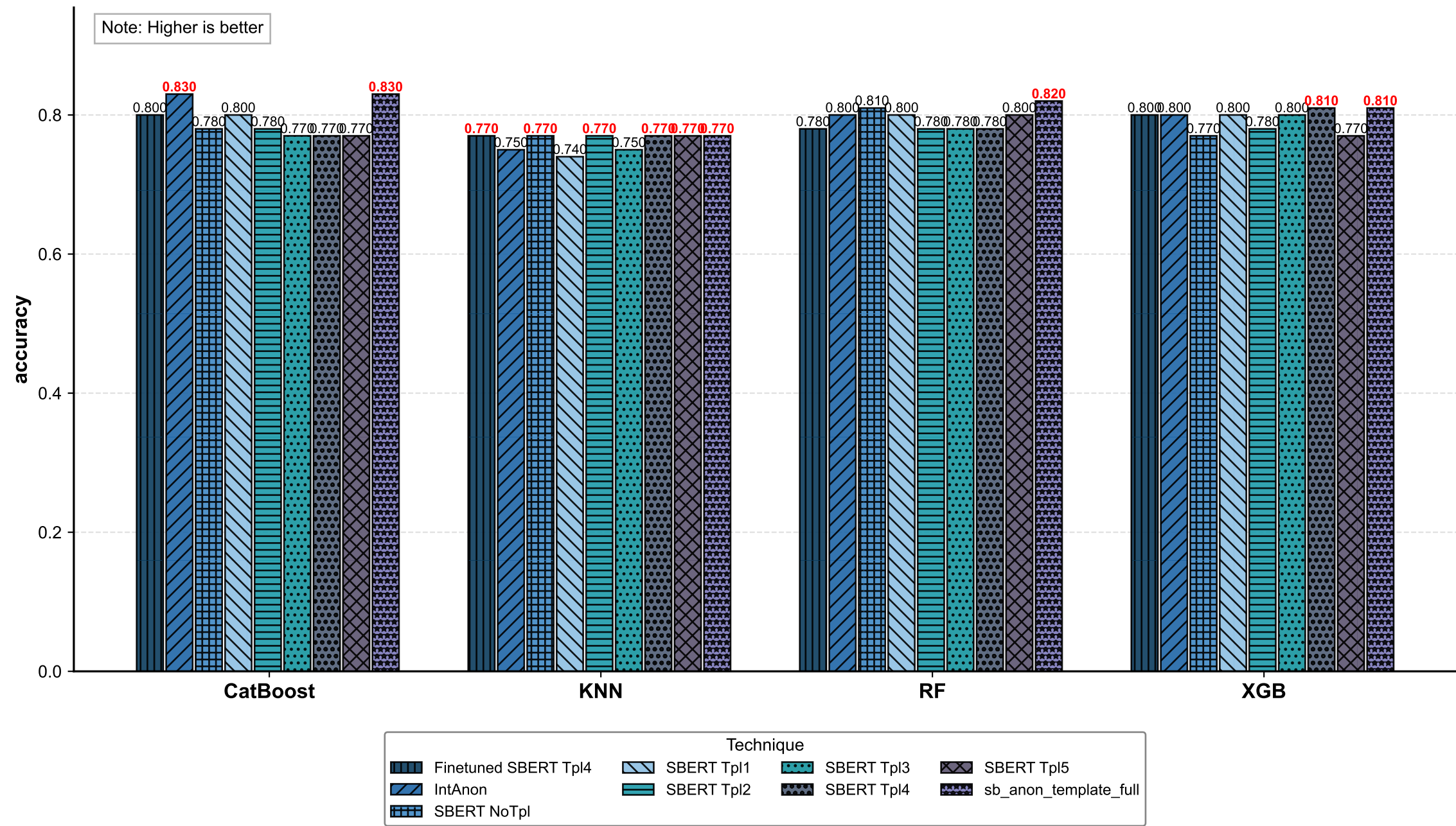
Task: job_state | Metric: accuracy
