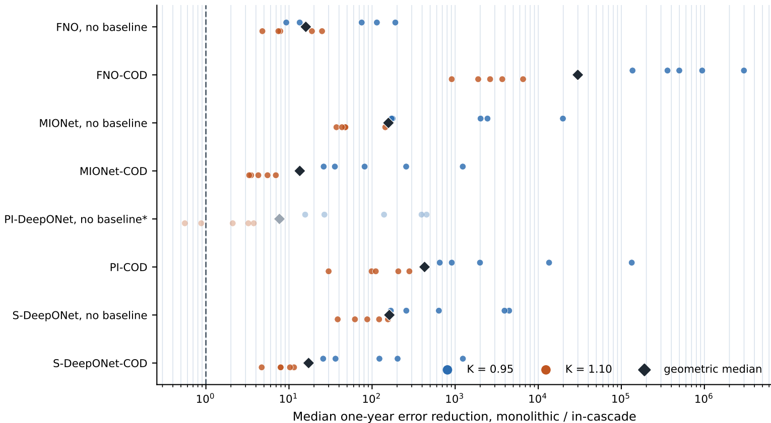
The cascade lowers long-horizon gas error across backbones
