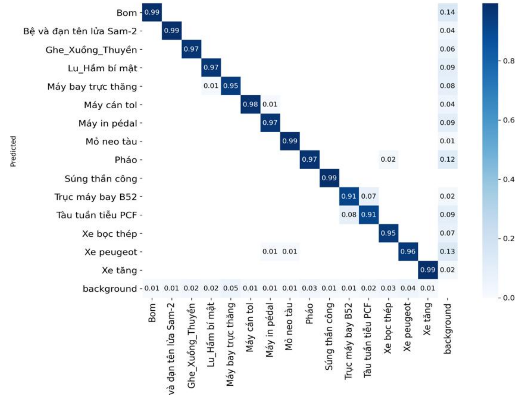
confusion_matrix_normalized_YoloV12s
