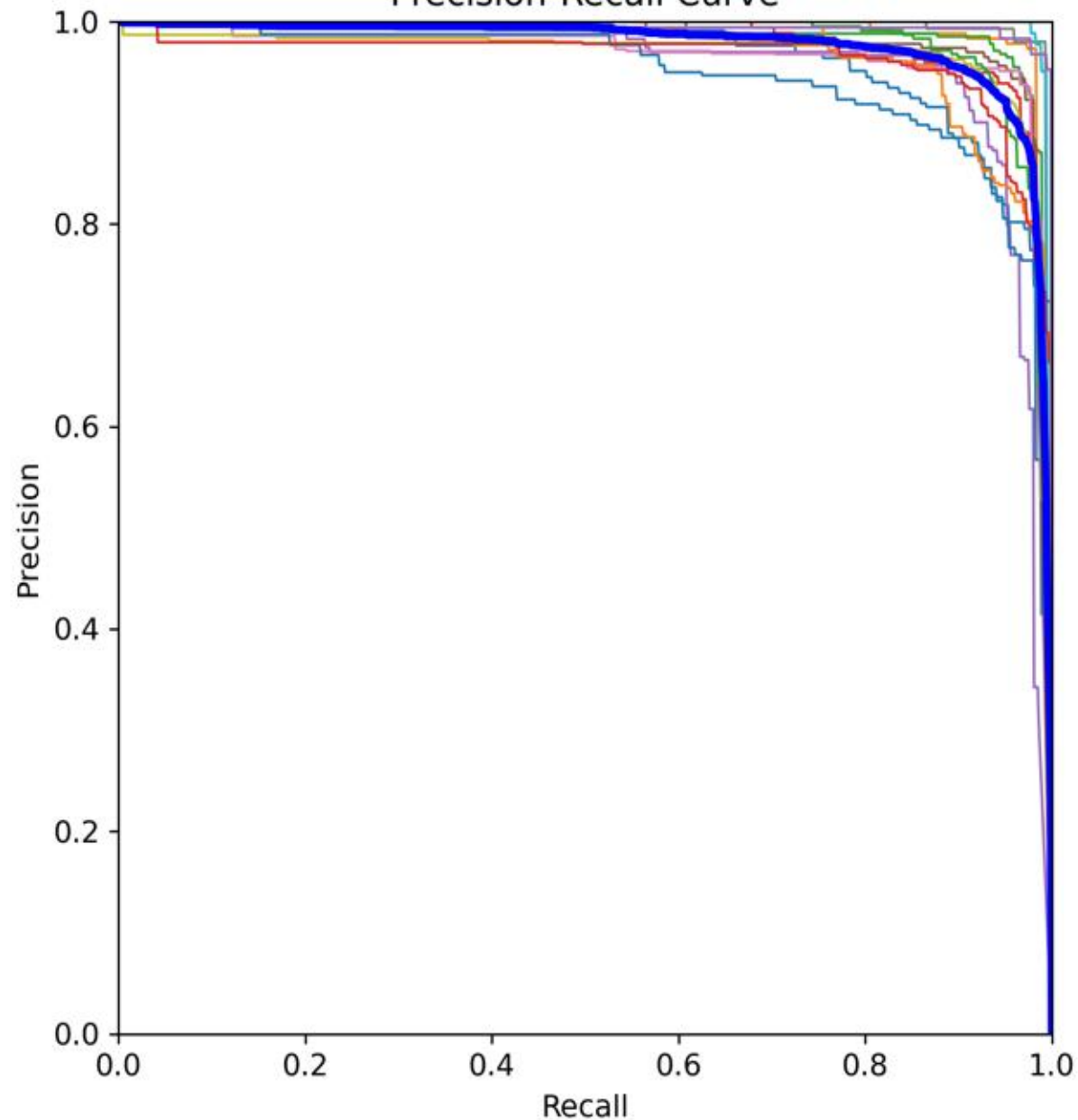
Precision-Recall Curve
