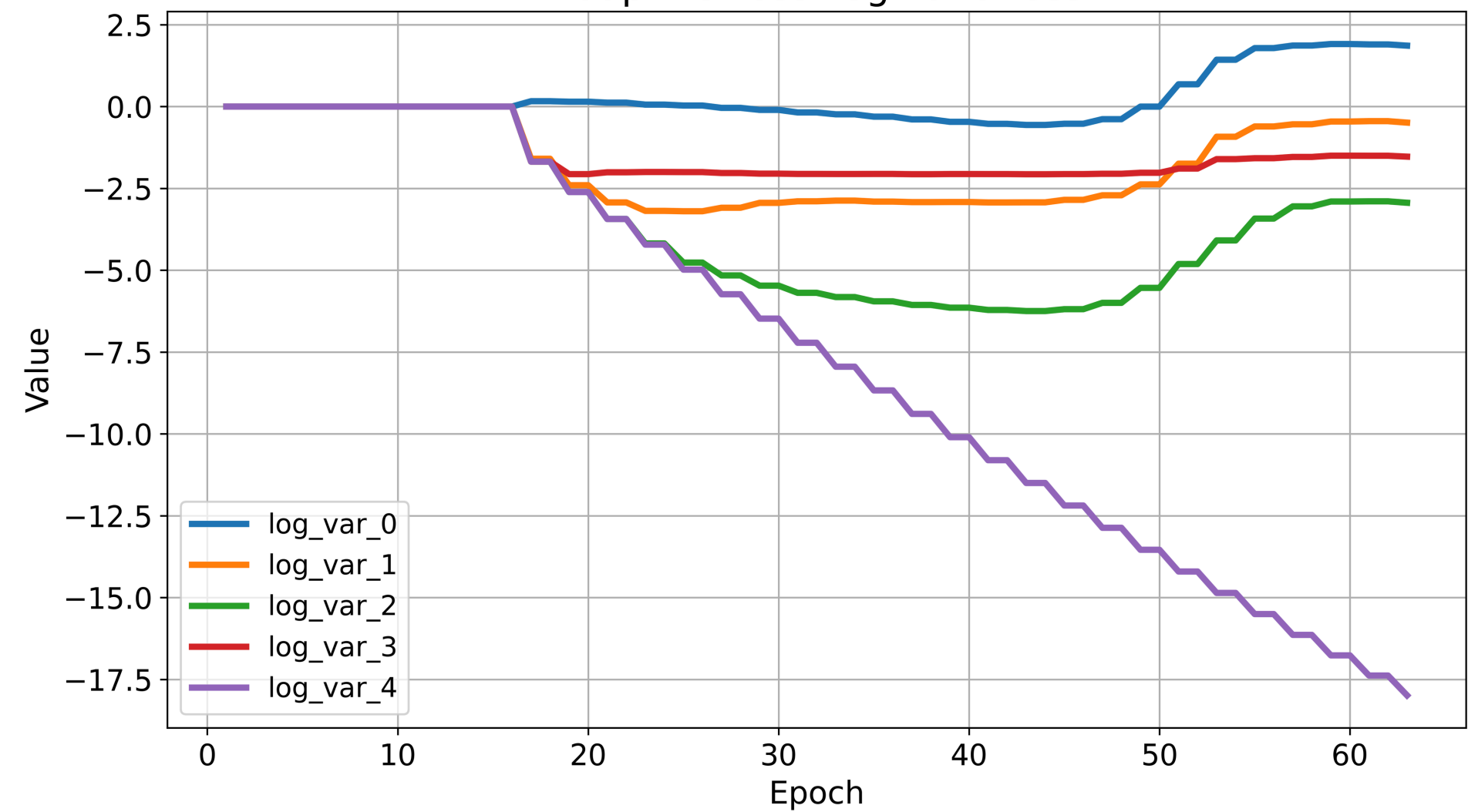
Adaptive Loss Log Variances
