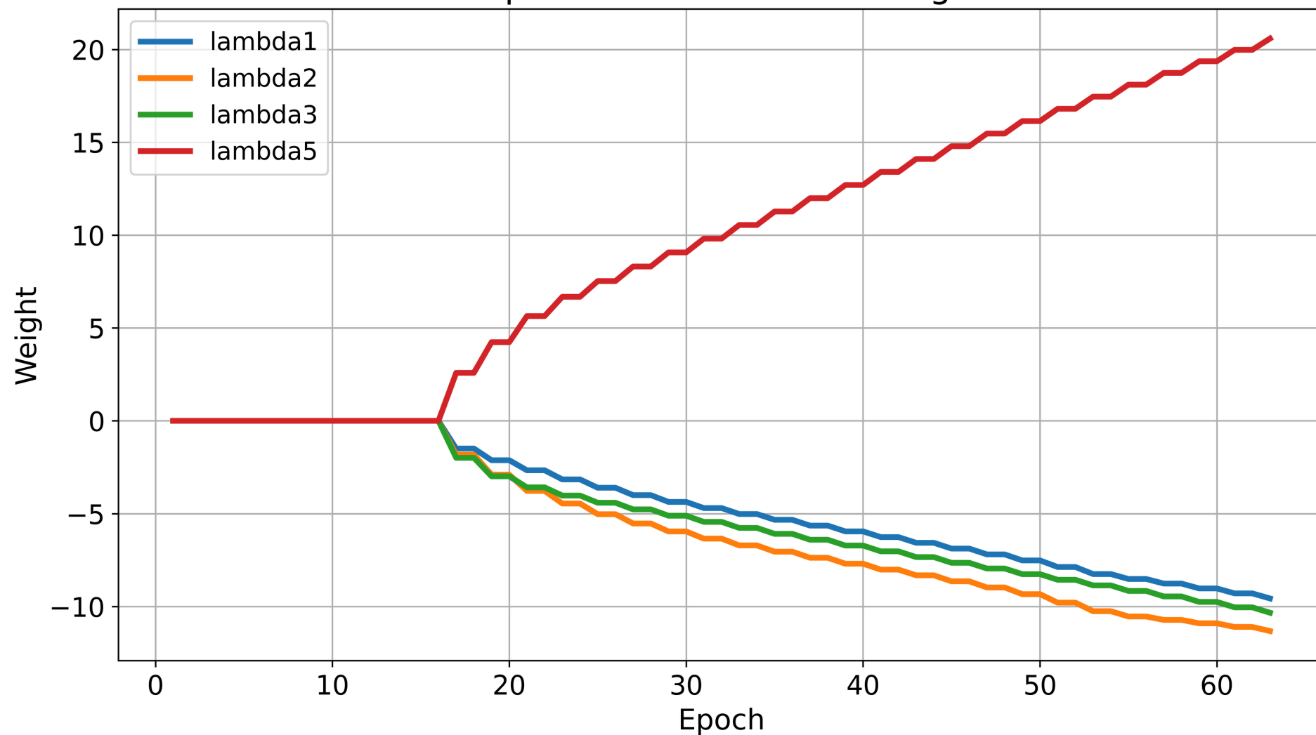
Prototype Learning Loss Components
