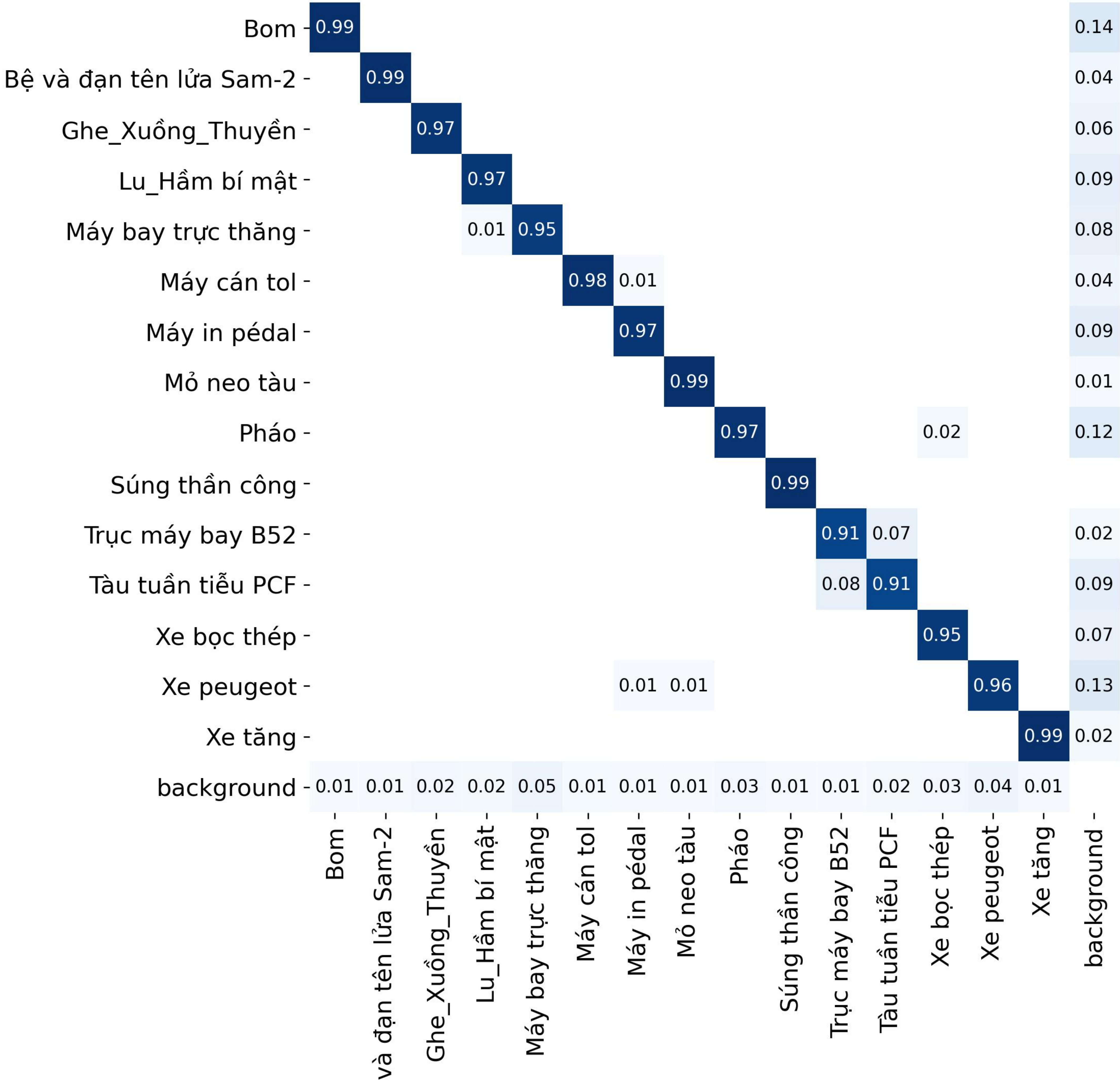
Confusion Matrix Normalized
