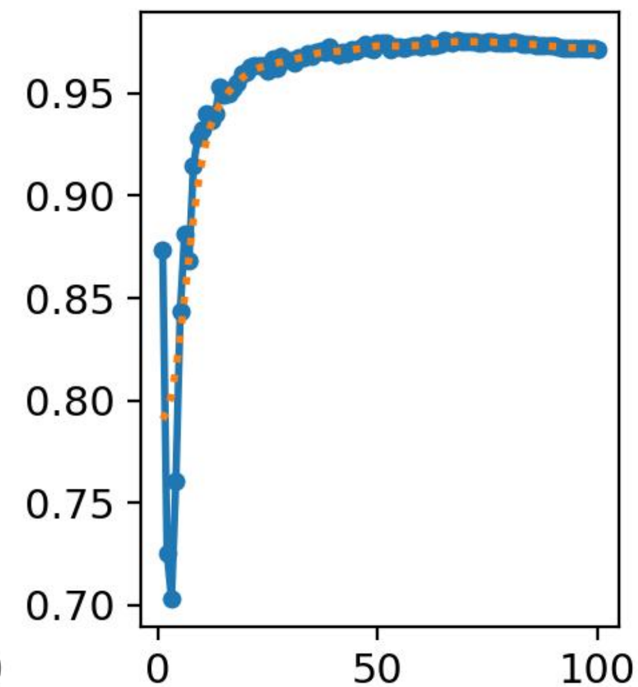
metrics/mAP50(B)
