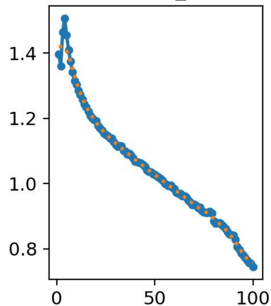
train/box_loss
