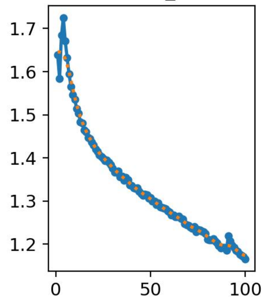
train/dfl_loss
