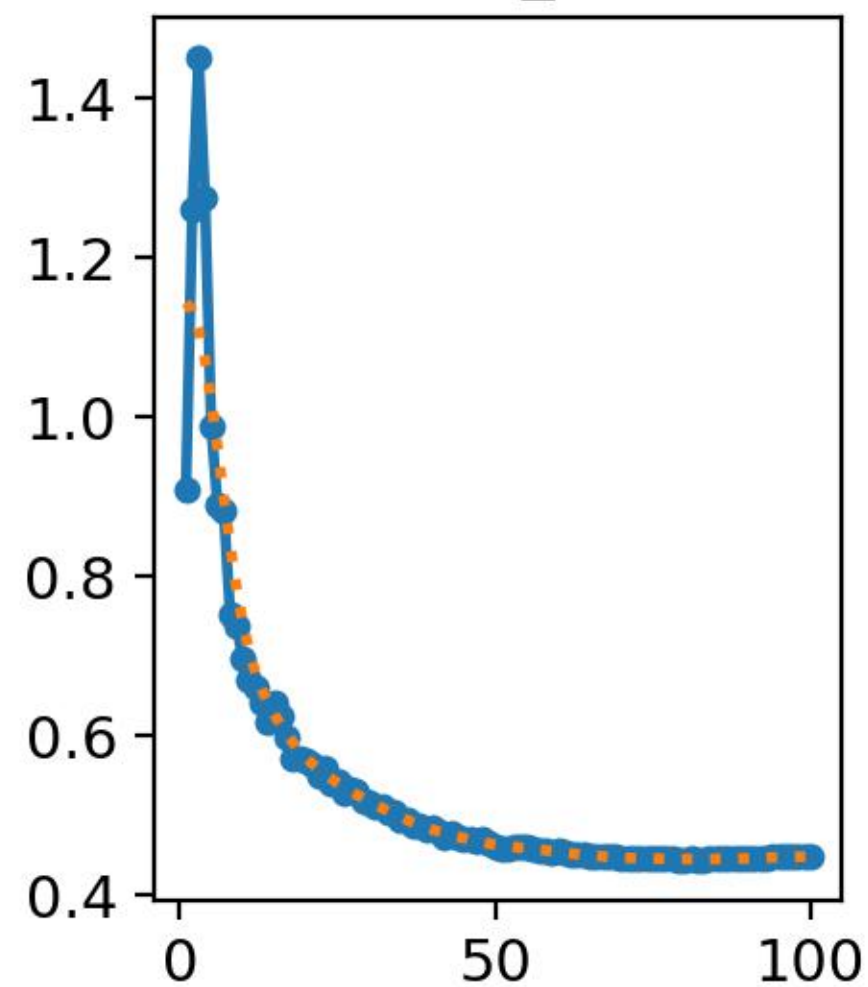
val/cls_loss
