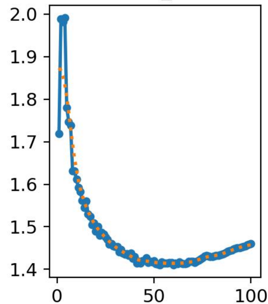
val/dfl_loss
