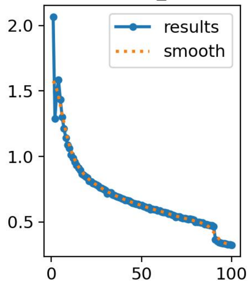
train/cls_loss
