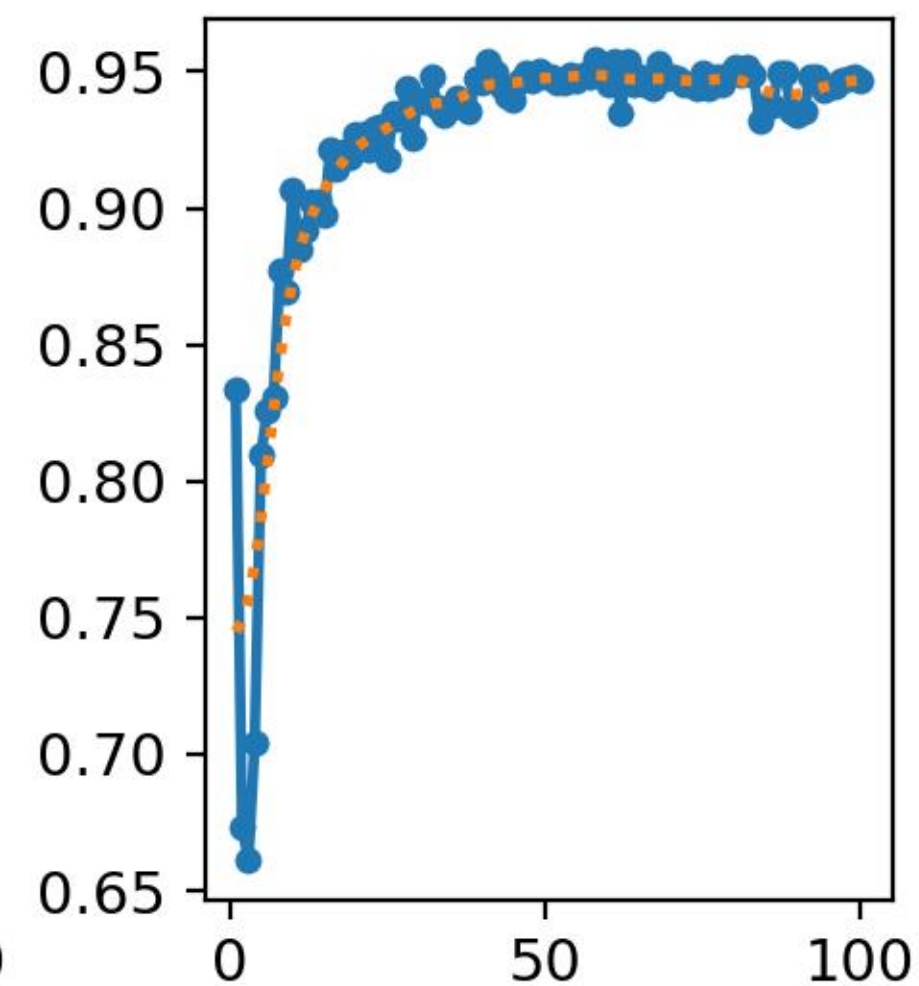
metrics/recall(B)
