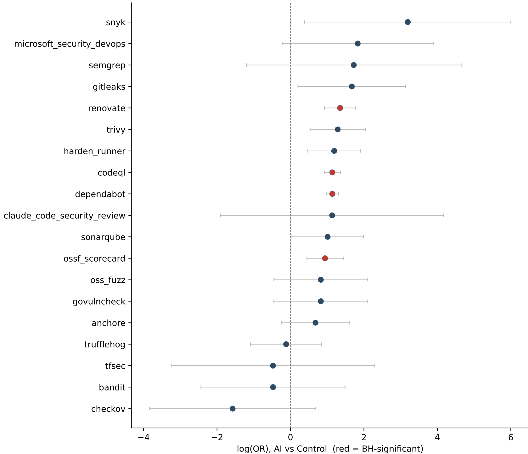
Per-tool odds ratios (Fisher's exact, BH within non-sparse subset)
