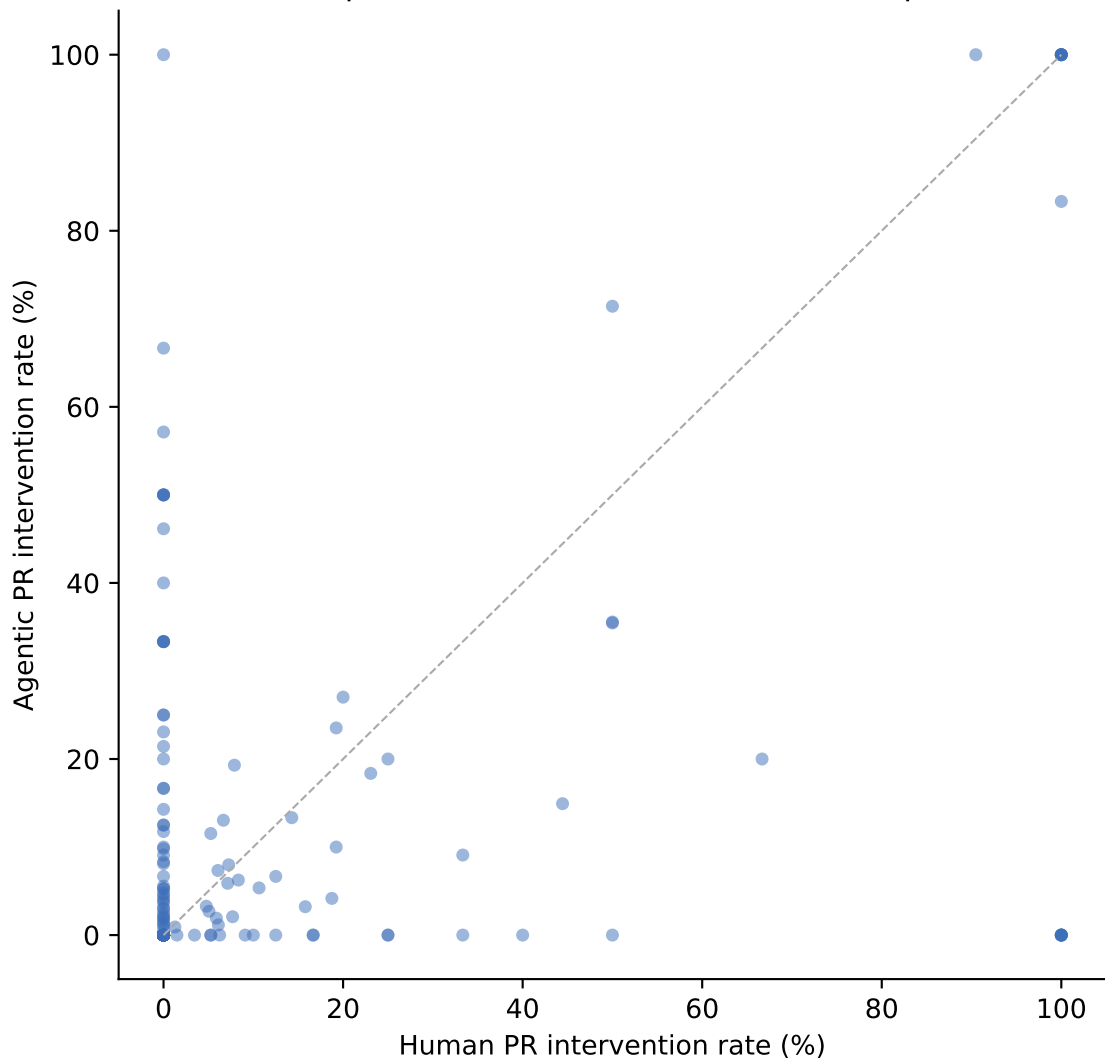
Per-repo intervention rates (n=588 FE repos)
