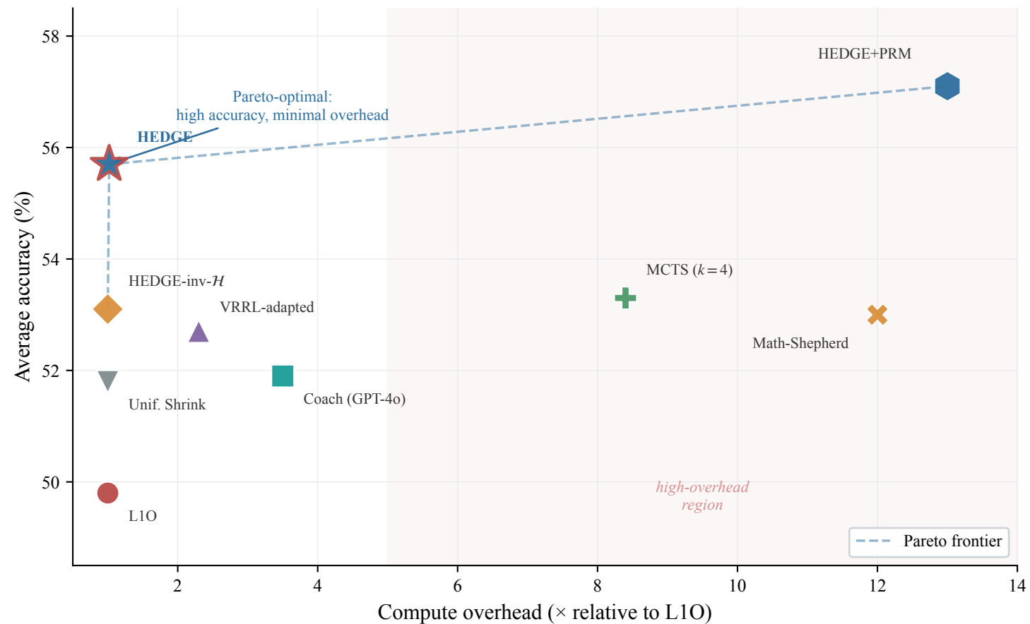
Compute-Performance Pareto Front ( n=8 , All Benchmarks)
