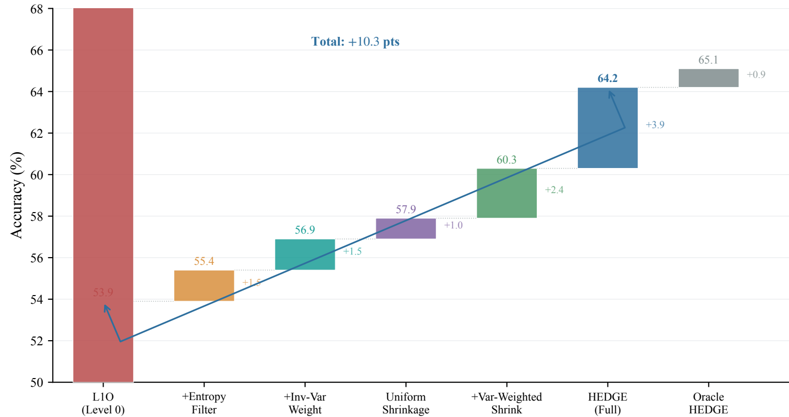
Six-Level Ablation: Component Contributions ( n = 12 , MathChat)
