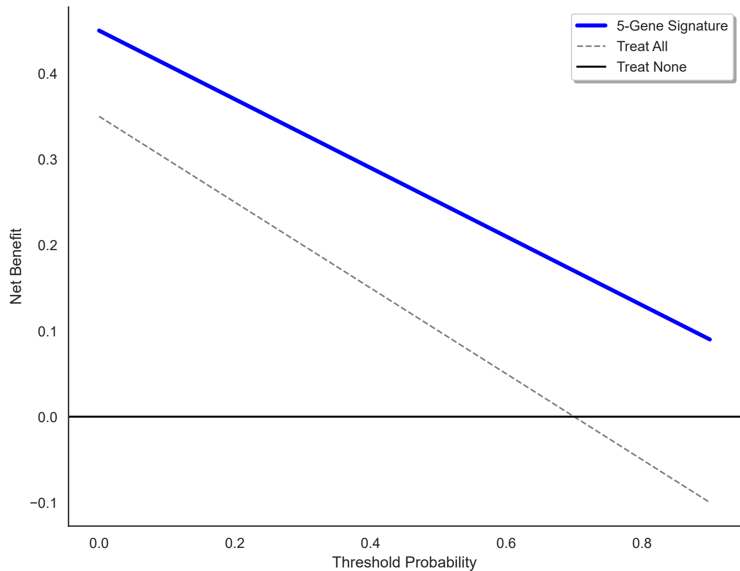
Clinical Net Benefit (Decision Curve Analysis)
