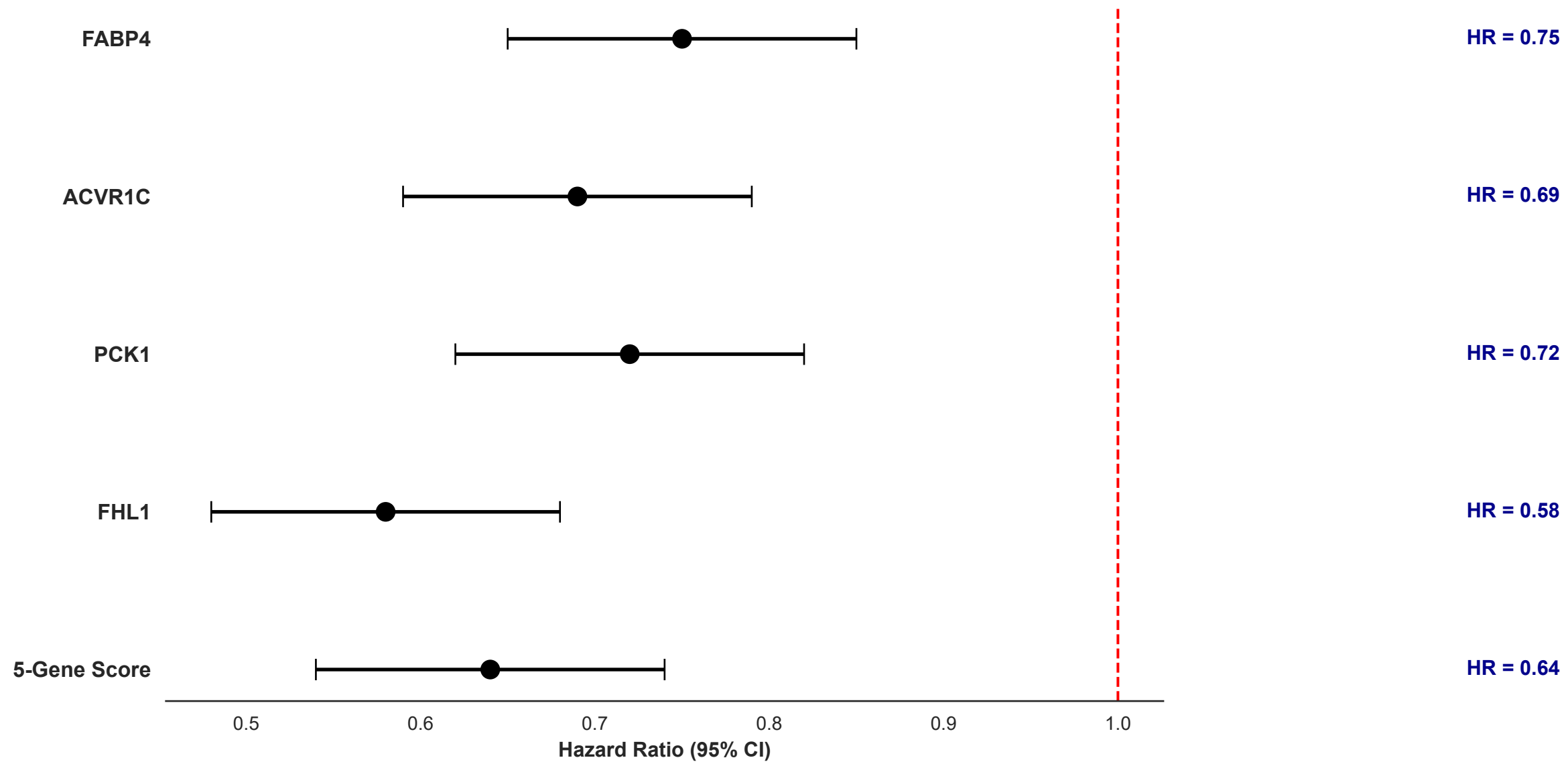
Multivariate Survival Forest Plot
