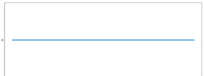
Duplicated Lines (%)
