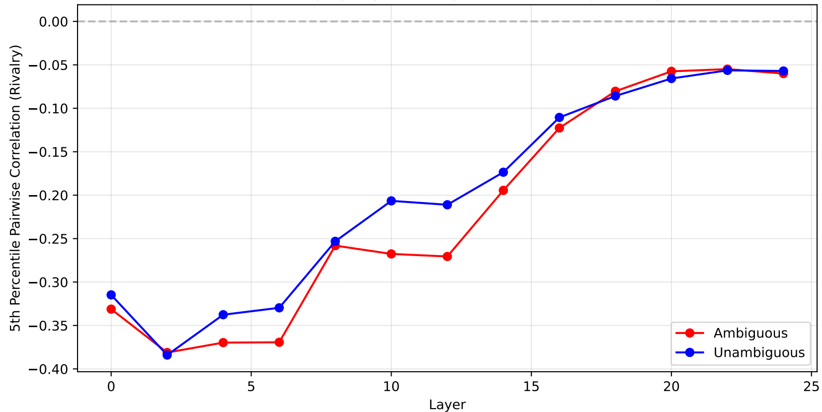
Feature Rivalry by Layer: Ambiguous vs Unambiguous Inputs
