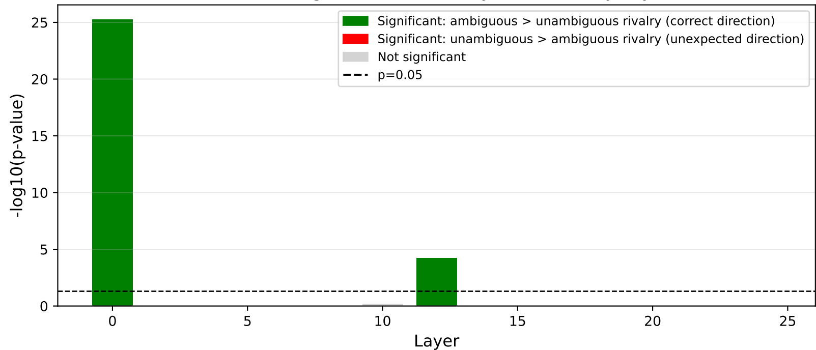
Statistical Significance of Rivalry Difference by Layer
