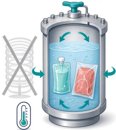
Isostatic HPP · chilled
