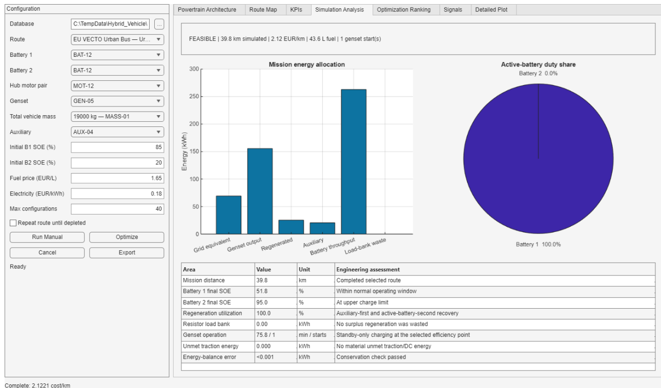
Figure 11.5. Simulation Analysis tab combining energy allocation, battery duty share, and engineering assessment
