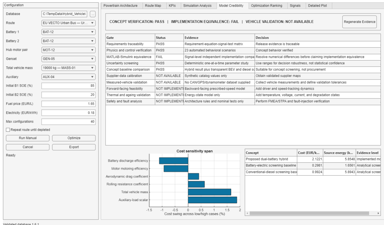
Figure 11.6. Model Credibility tab separating verified concept behavior from open implementation and validation gates
