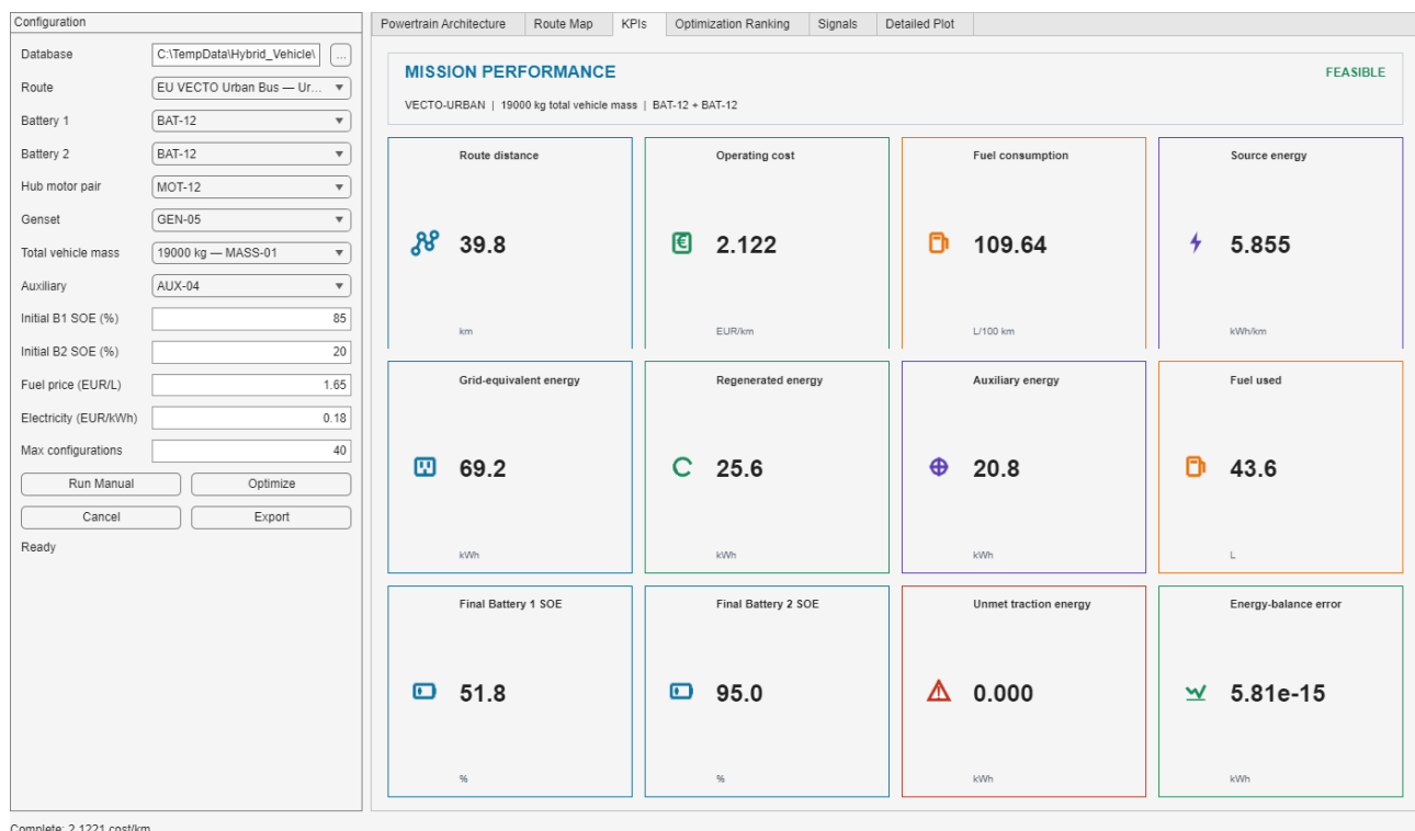
Figure 11.4. Management KPI dashboard with icon-led values, units, configuration context, and feasibility status
