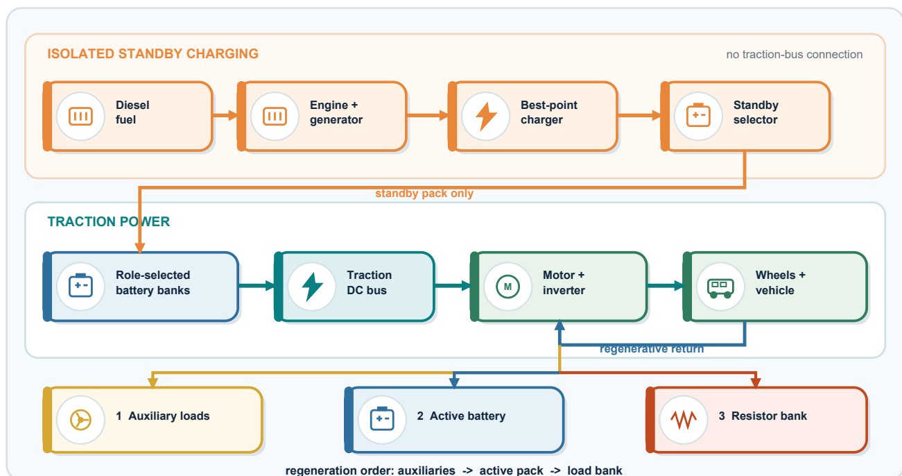
Figure 2.1. Conceptual energy flow, isolated genset path, and regeneration priorities
