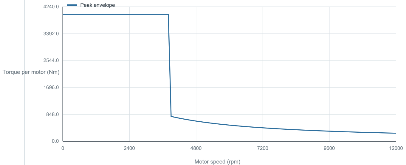
Figure 5.1. Selected motor constant-torque and constant-power regions
