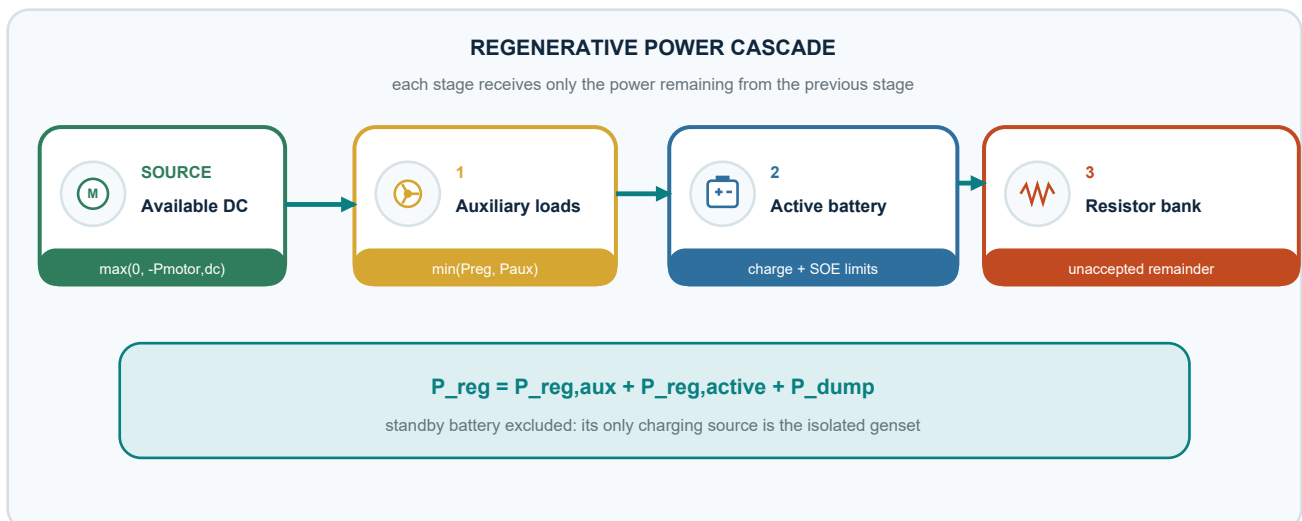
Figure 8.2. Strict auxiliary-active-battery-resistor regeneration hierarchy
