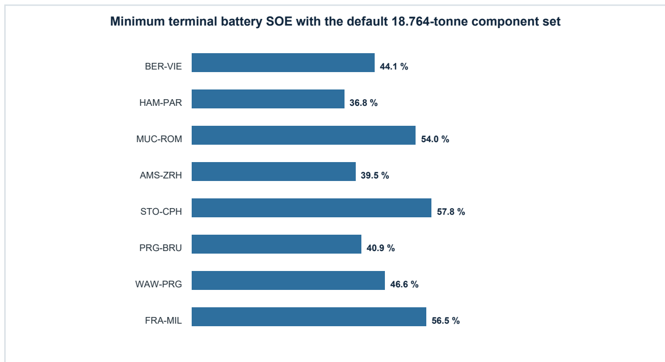
Figure 16.2. Minimum terminal pack SOE after one prescribed long-route pass
