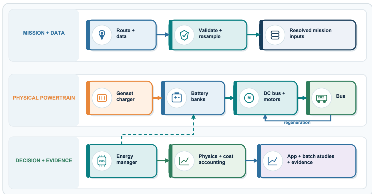
Figure 1.1. End-to-end project architecture from sourced routes to app, batch-study, and evidence outputs
