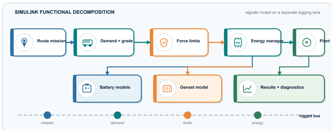
Figure 2.2. Readable Simulink subsystem decomposition and separated logging lane
