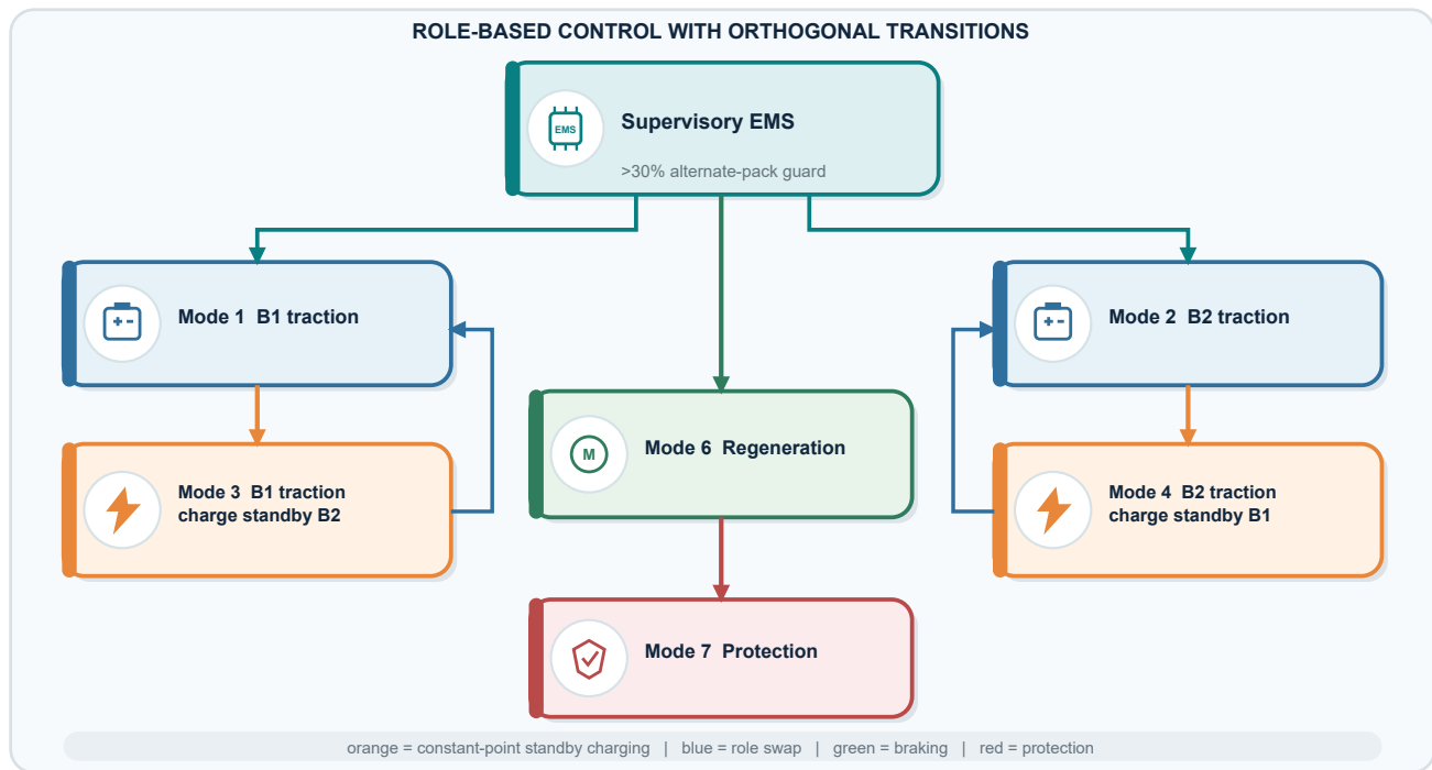
Figure 8.1. Supervisory operating modes and principal transitions
