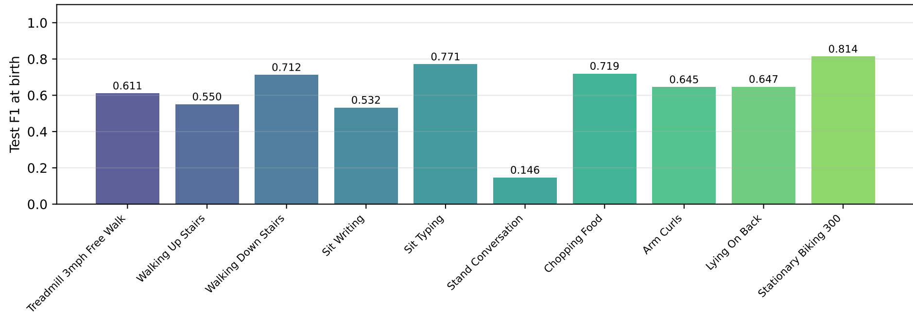
New Activity Head F1 at Birth (2-stream, real data)
