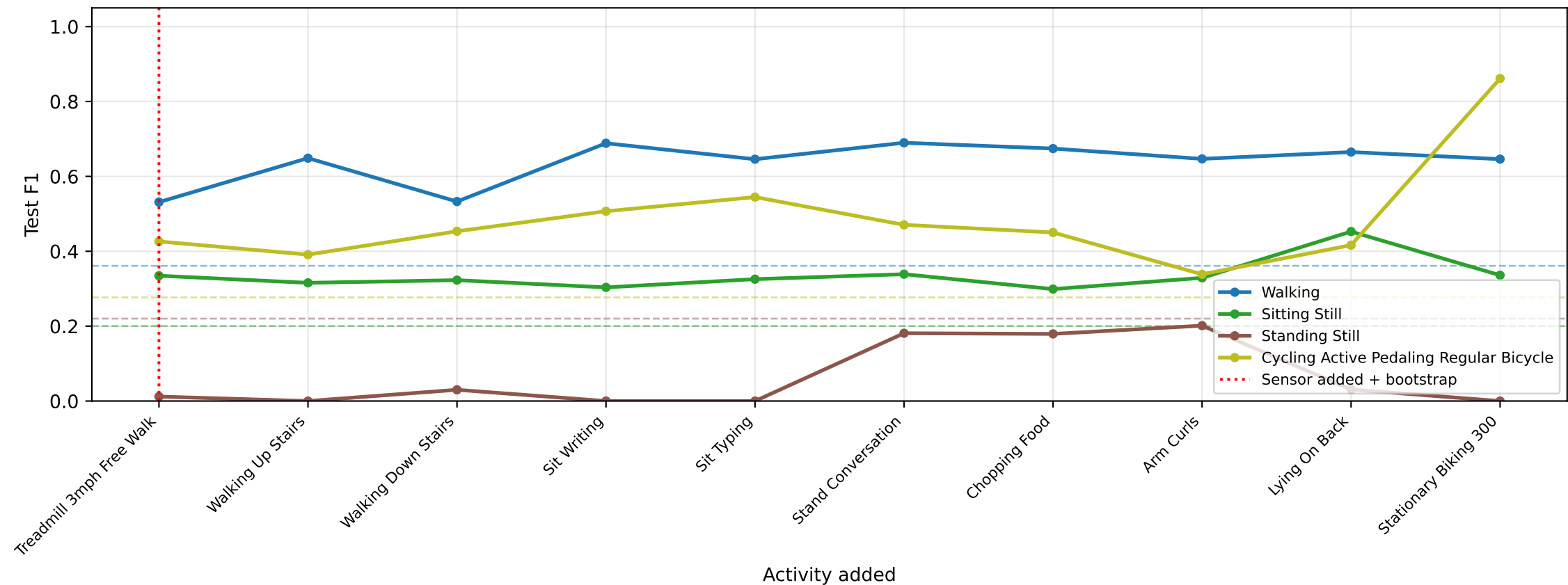
Seed Head F1 Progression (dashed = E1 baseline on 1-stream; solid = after sensor increment)
