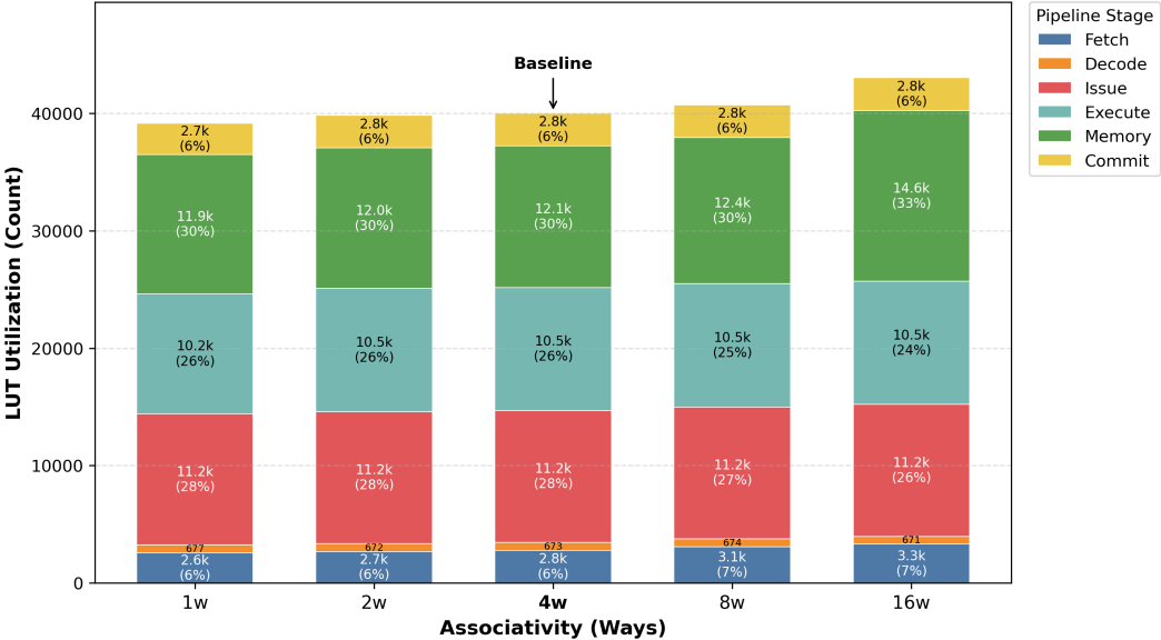
Associativity Sweep: LUT Distribution
