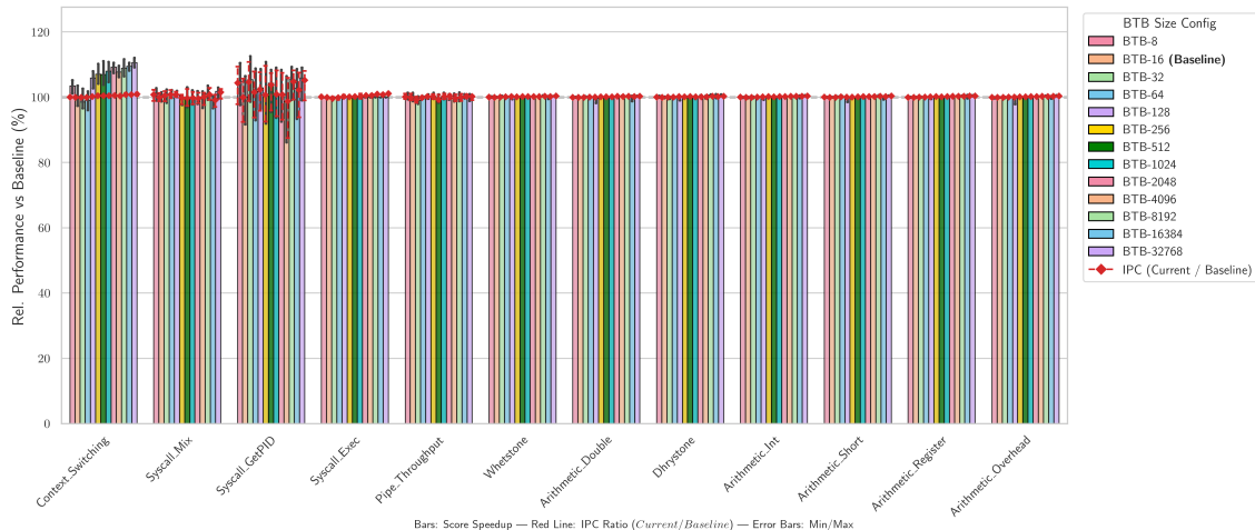
UnixBench Suite: Sensitivity to BTB Size
