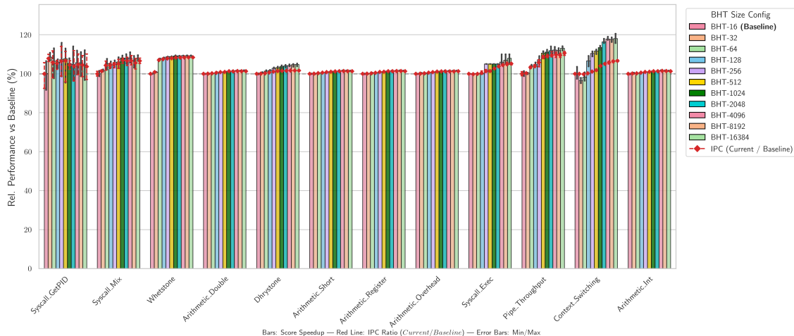
UnixBench Suite: Sensitivity to BHT Size
