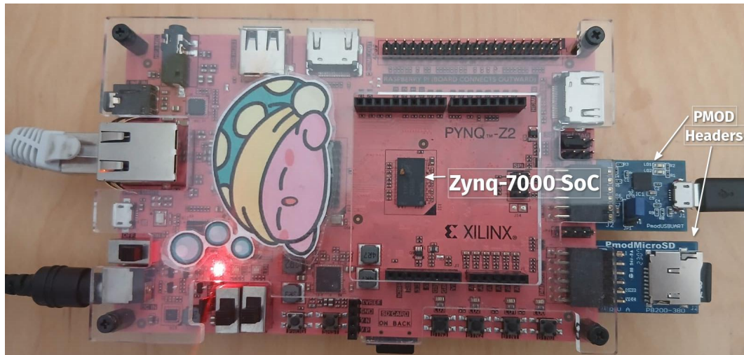
CVA6 Single Core deployment on a PYNQ-Z2 FPGA with PMod Modules
