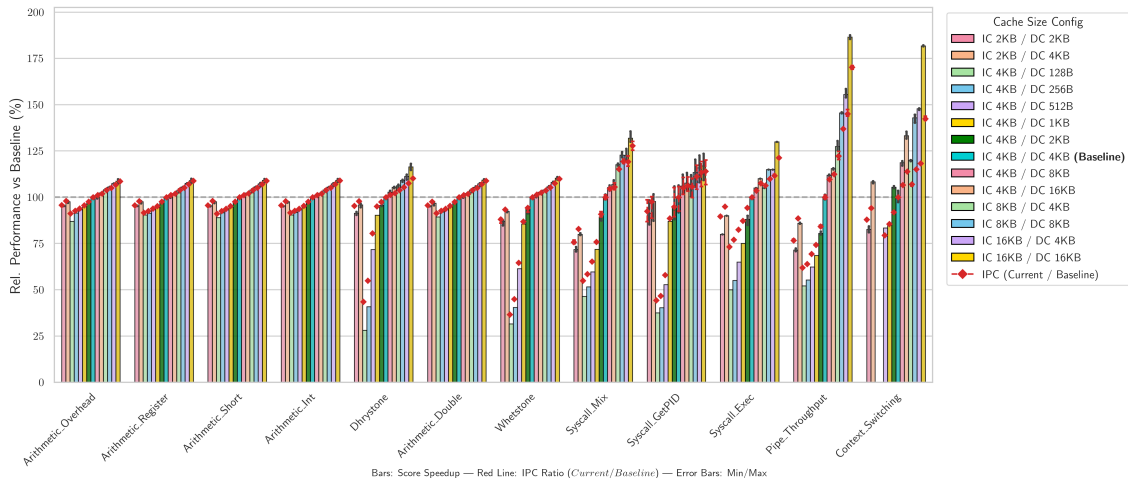
UnixBench Suite: Sensitivity to Cache Size
