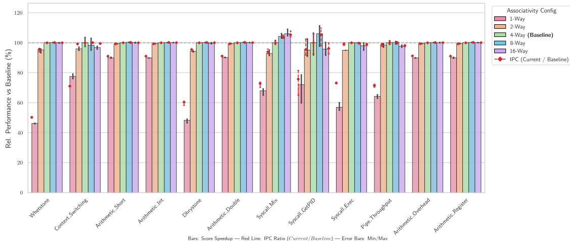
UnixBench Suite: Sensitivity to Associativity
