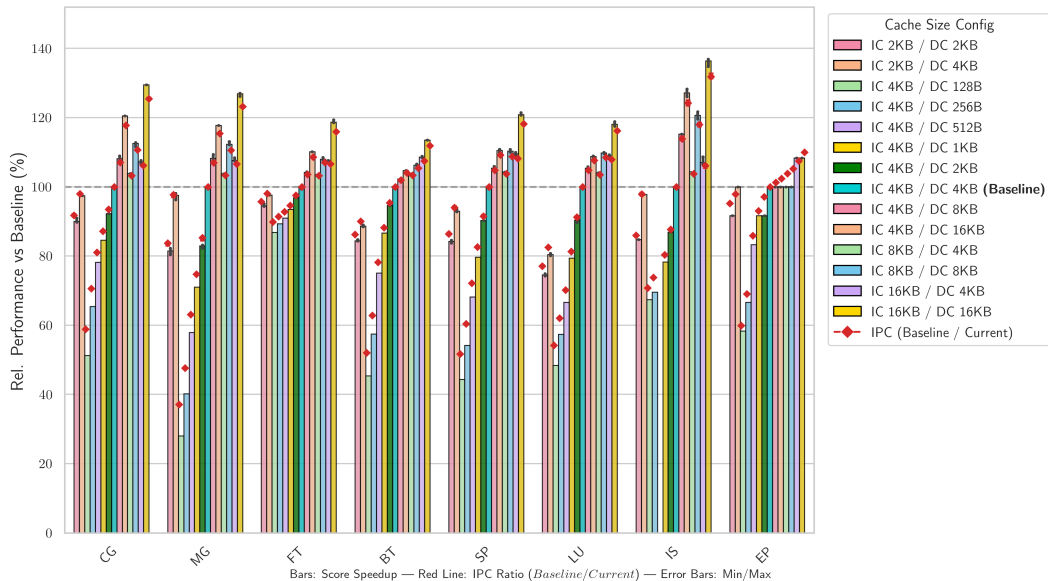
NPB Suite: Sensitivity to Cache Size
