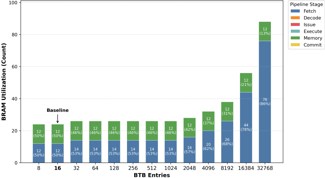
BTB Size Sweep: BRAM Distribution
