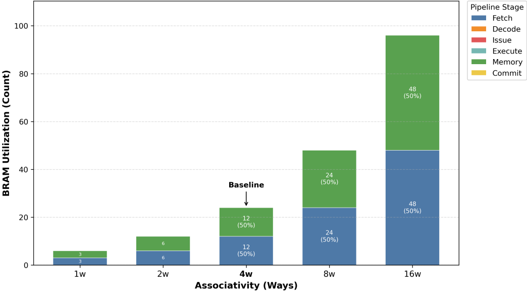
Associativity Sweep: BRAM Distribution
