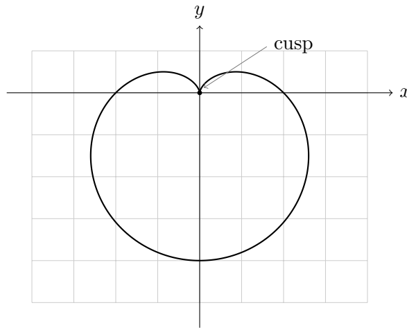
The cardioid r = 1 - \sin \theta (that is, a = 1 ).
