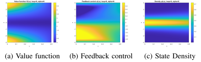
Fig. 1: (a)-(c): Simulations results for a GMFG with time varying control constraints that depends on \bar{\lambda}_\alpha
