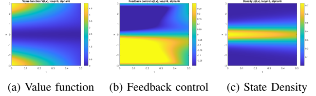
Fig. 2: (a)-(c): Simulations results for a GMFG with an universal control constraints
