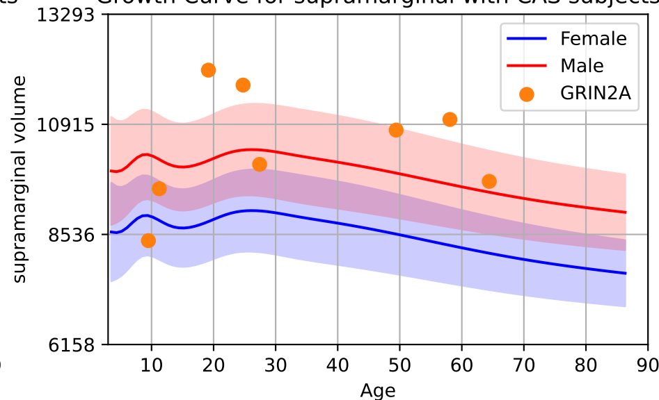
Growth Curve for supramarginal with CAS subjects
