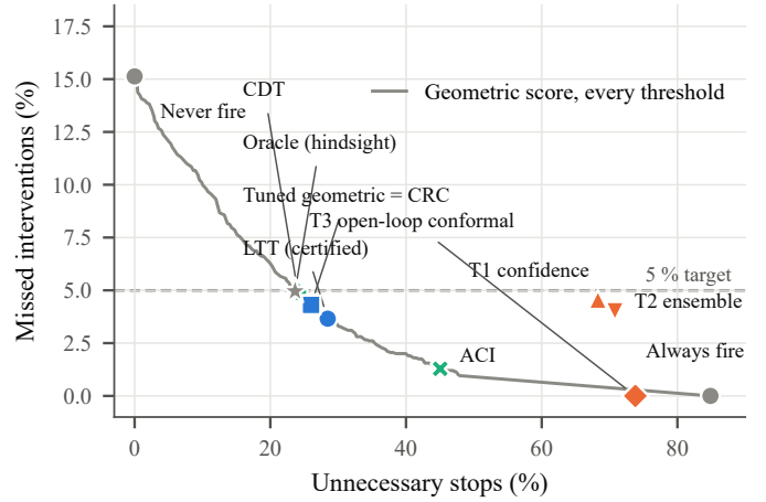
Fig. 2. Every method at its operating point (Table I), against the geometric score’s own miss-versus-stops curve as its threshold varies. On this split most methods sit below the dashed \alpha = 0.05 line; the geometric methods do so at well under half the stops of the confidence, ensemble and open-loop triggers. Which of them keeps the target across resplits is shown in Fig. 3.
