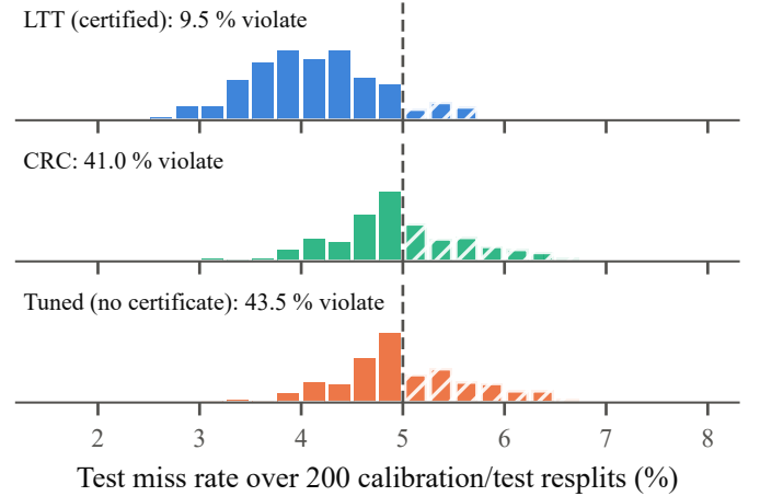
Fig. 3. Test miss rate over 200 calibration/test resplits. Dashed line: the 5 % target; hatched bars: resplits that violate it. A valid certificate keeps violations at or below \delta = 10 %. LTT’s high-probability guarantee does (9.5 %); CRC’s expectation guarantee and empirical tuning do not.
