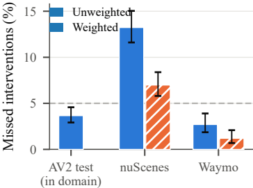
(a) Threshold certified on AV2
