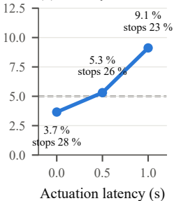
(b) Latency, AV2 test
