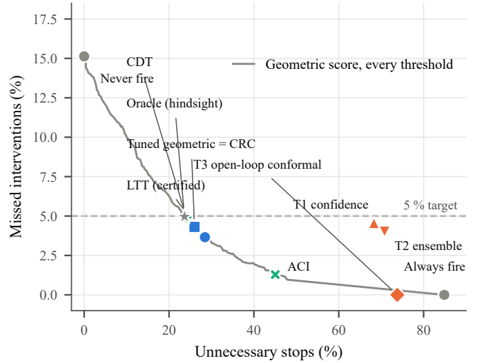
Fig. 1. Every method at its operating point (Table II), against the geometric score's own miss-versus-stops curve as its threshold varies. Only points below the dashed target line meet \alpha = 0.05 ; only LTT does so while also staying close to the curve's lower envelope.
