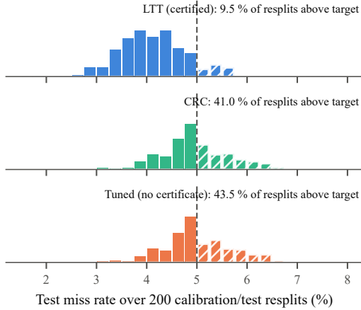
Fig. 2. Test miss rate over 200 calibration/test respits. LTT’s high-probability guarantee keeps violations at 9.5 %; CRC’s expectation guarantee and empirical tuning do not.
