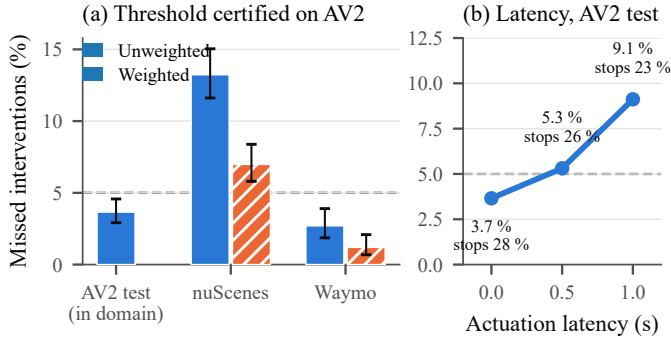
Fig. 3. (a) Miss rate of the Argoverse 2-certified threshold deployed unchanged on nuScenes and Waymo, unweighted and with the density-ratio repair (Section III-D); error bars are 95 % Wilson CIs. (b) Miss rate and unnecessary stops as actuation latency increases (Table IV).
