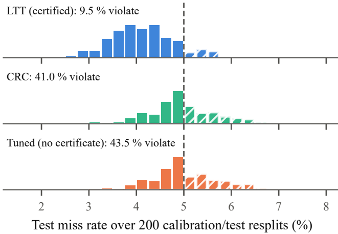
Fig. 3. Test miss rate over 200 calibration/test resplits. Dashed line: the 5% target; hatched bars: resplits that violate it. A valid certificate keeps violations at or below \delta = 10\% . LTT's high-probability guarantee does (9.5%); CRC's expectation guarantee and empirical tuning do not.
