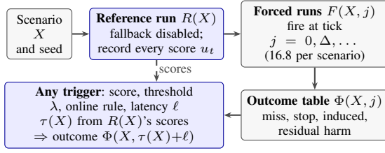
Fig. 1. Lookup evaluation (Observation 1). One reference run and one forced rollout per decision tick are simulated once per scenario. Every trigger, threshold, online update rule and latency is then evaluated by lookup on identical physics, instead of one rollout per combination (over 7,000 per scenario here).
