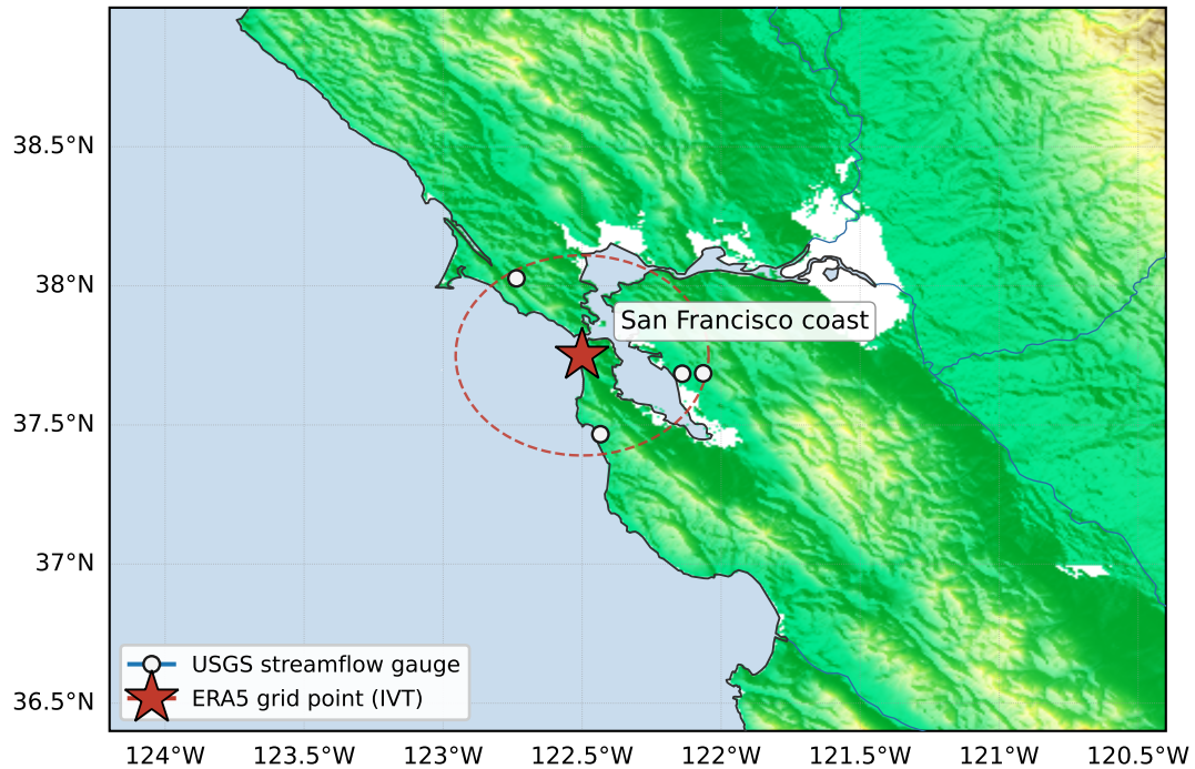
(a) California 37.75°N, 122.50°W IVT threshold 249.8 kg m -1 s -1
