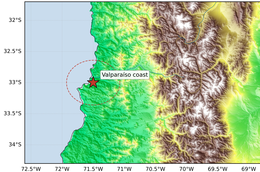
(b) Central Chile 33.00°S, 71.50°W IVT threshold 161.8 kg m -1 s -1
