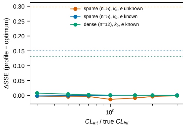
Multi-start (6 restarts)
