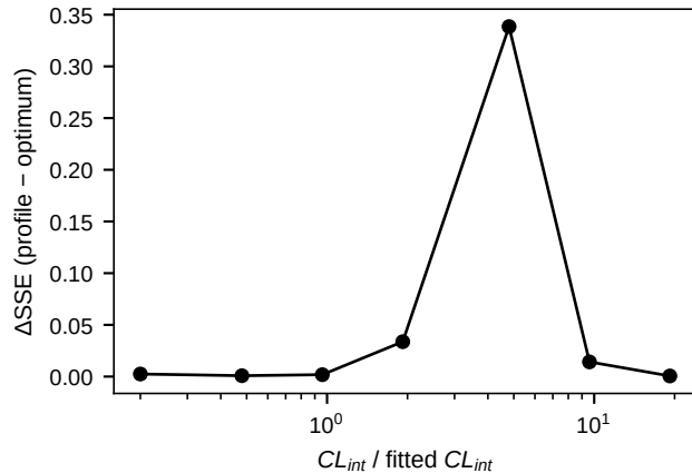
Single-start (naive)
