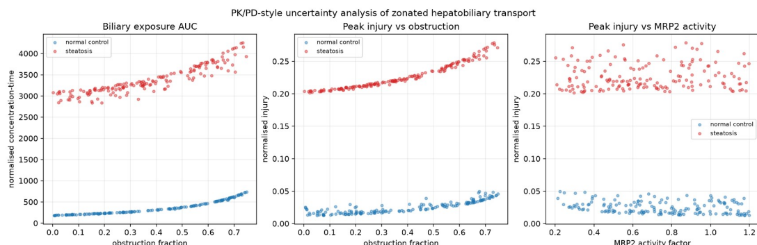
Figure 2. Exposure and injury sensitivity to obstruction-like stress and MRP2 activity. The outputs are normalized and intended for model qualification, not clinical dosing.
