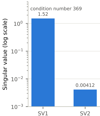
Local Jacobian, rank 2 of 6 parameters
