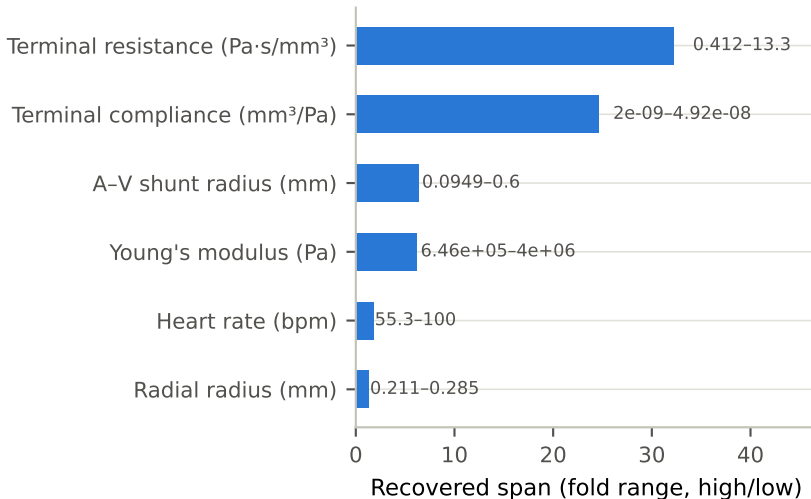
Synthetic inverse recovery, 20 starts
