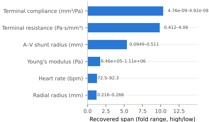
Synthetic inverse recovery, 3 starts
